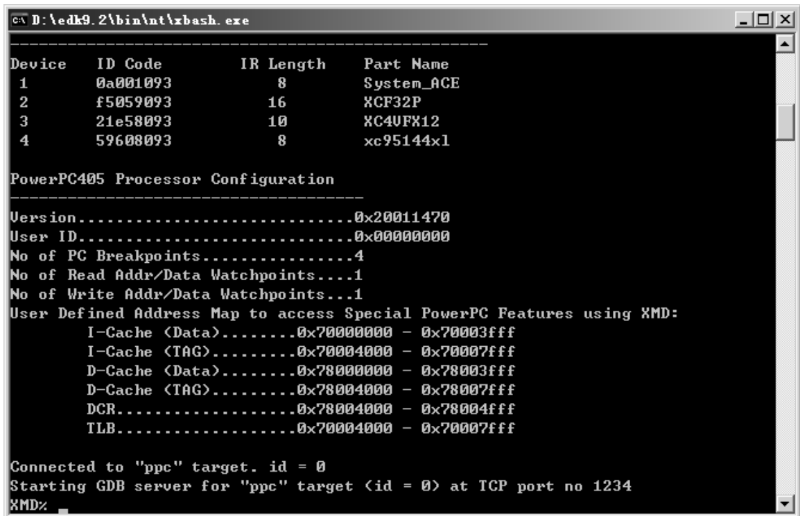
Figure 32: XMD Window
