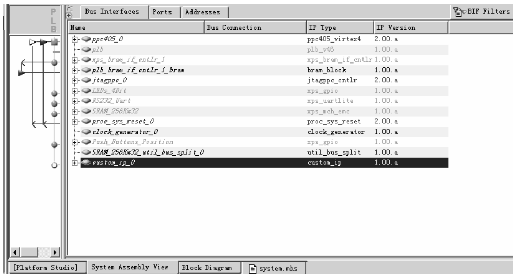
Figure 19: Inserting IP
