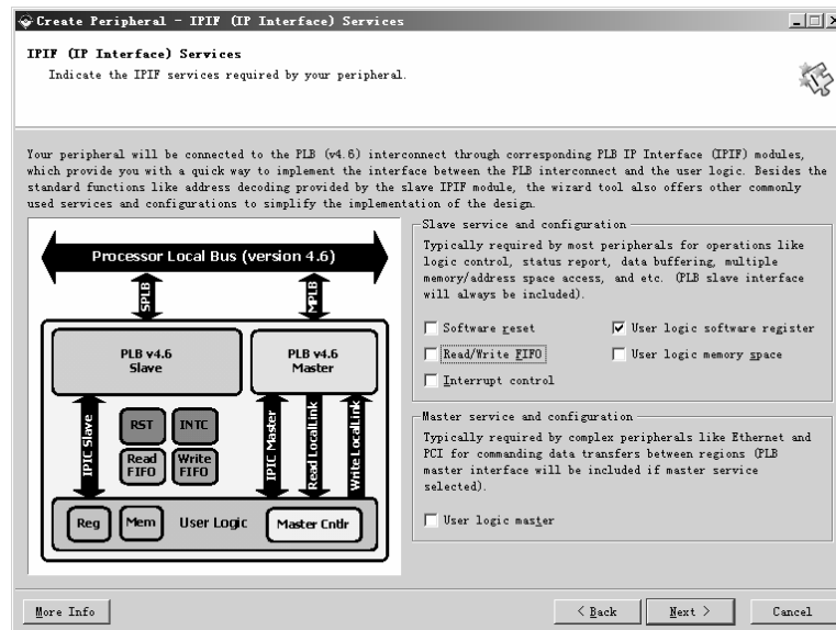
Figure 15: Create Peripheral - IPIF Services
