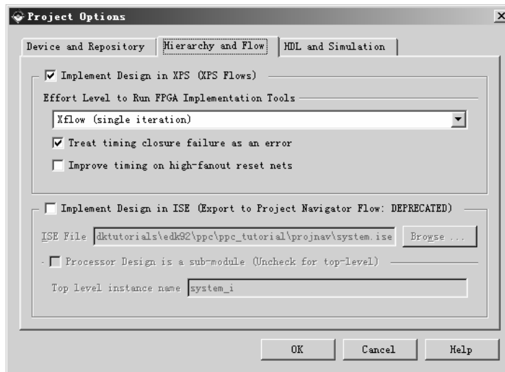
Figure 13: Project Options - Hierarchy and Flow
