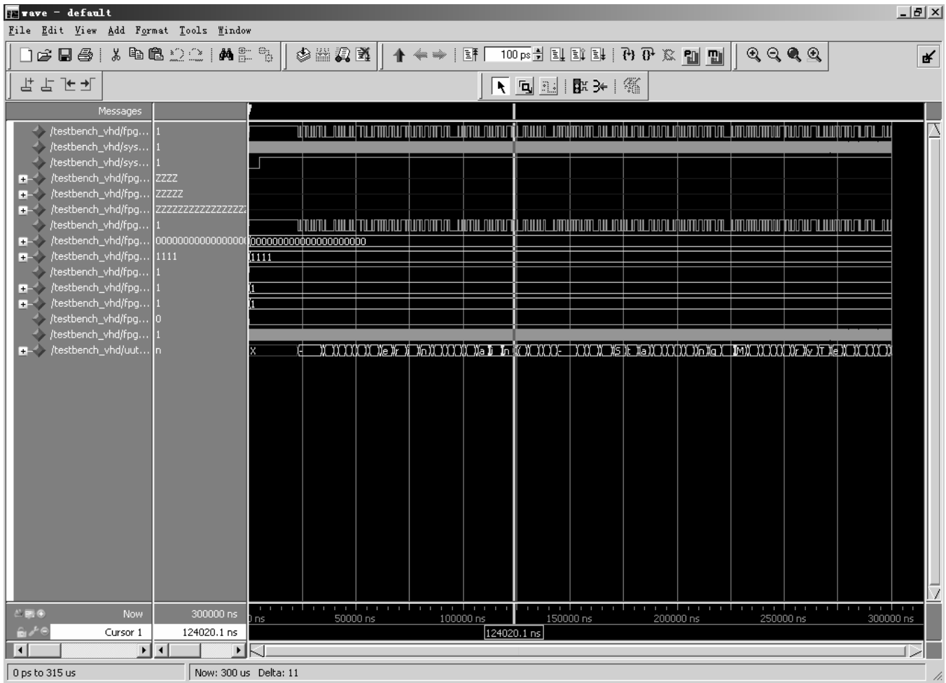
Figure 38: Simulation results
