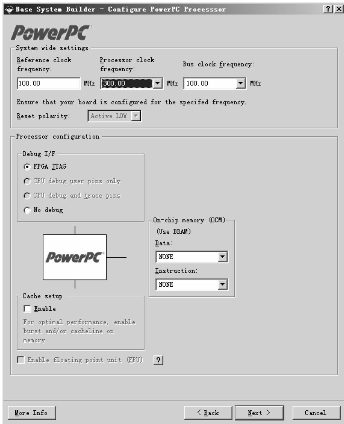
Figure 3: Configure Processor
