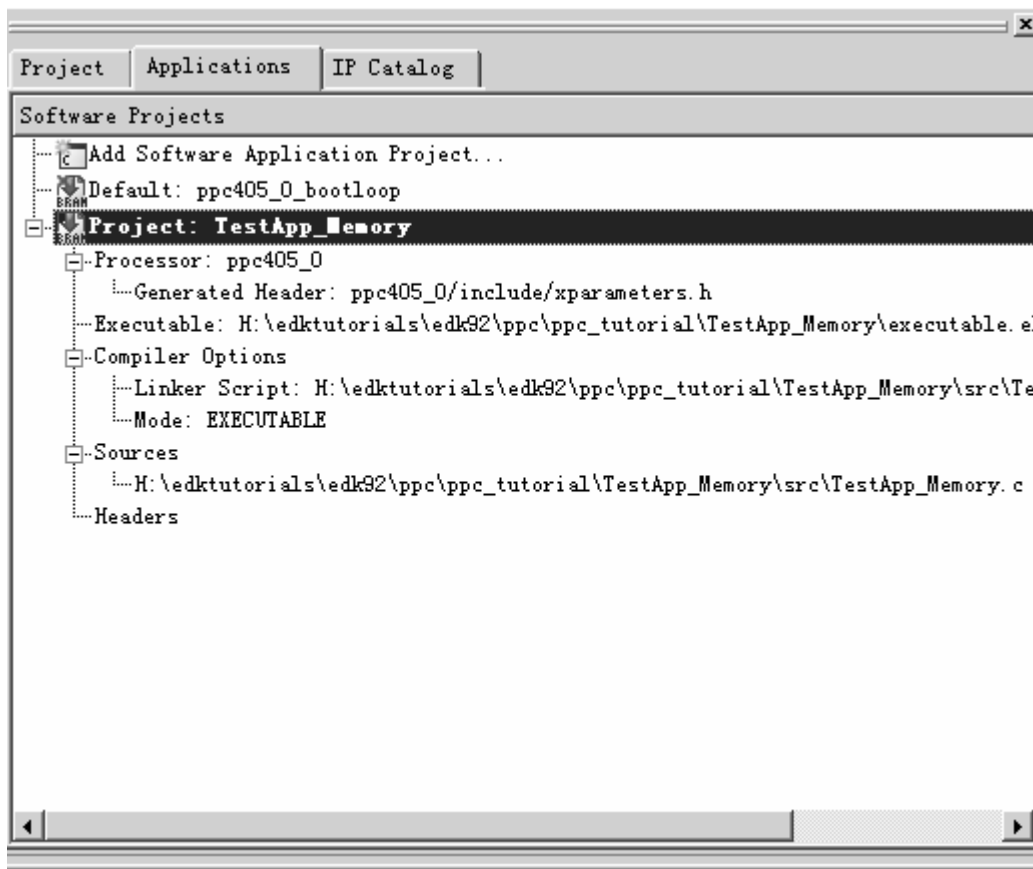
Figure 29: Applications Tab
