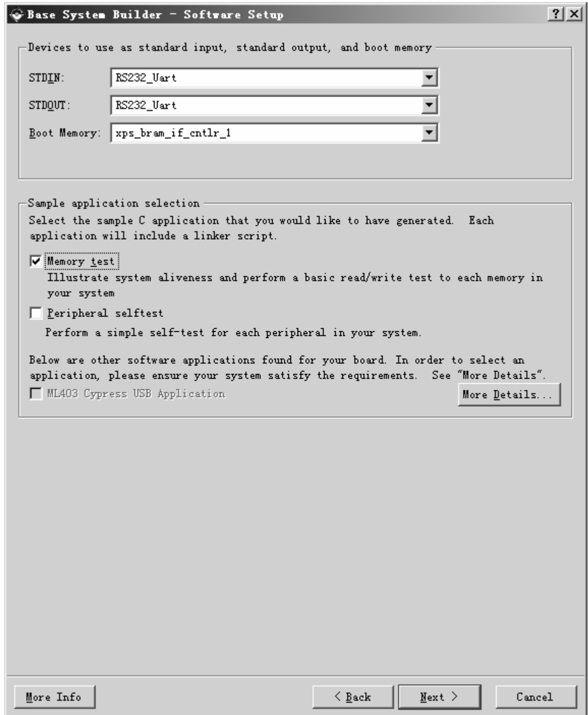
Figure 8: Software Setup
