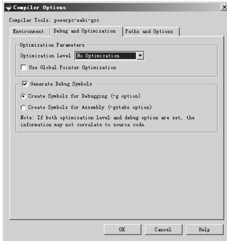
Figure 34: Compiler Options
