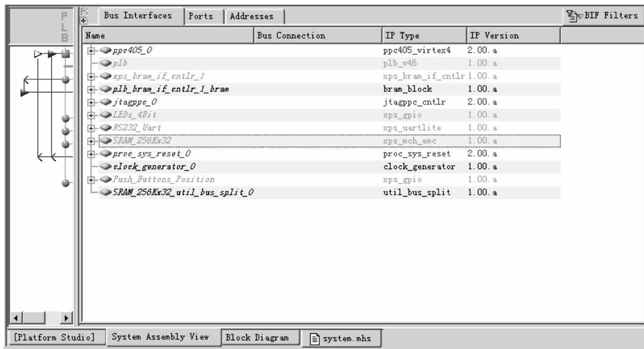
Figure 18: System Assembly View
