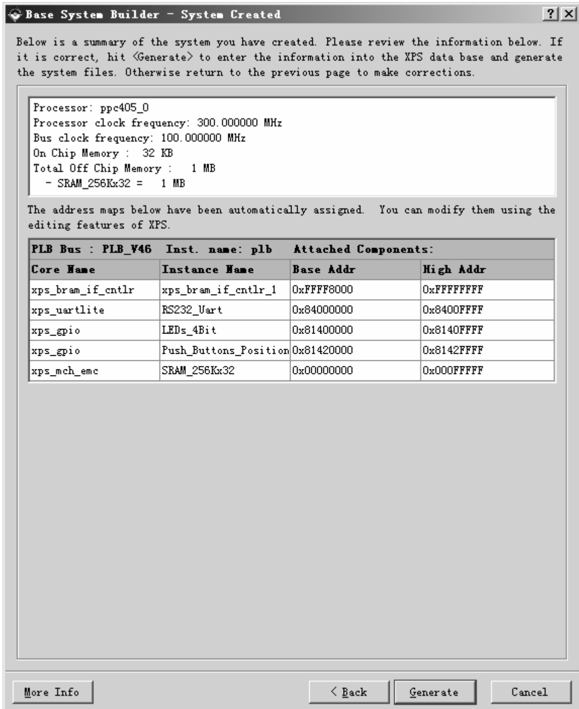
Figure 10: Completed Processor System
