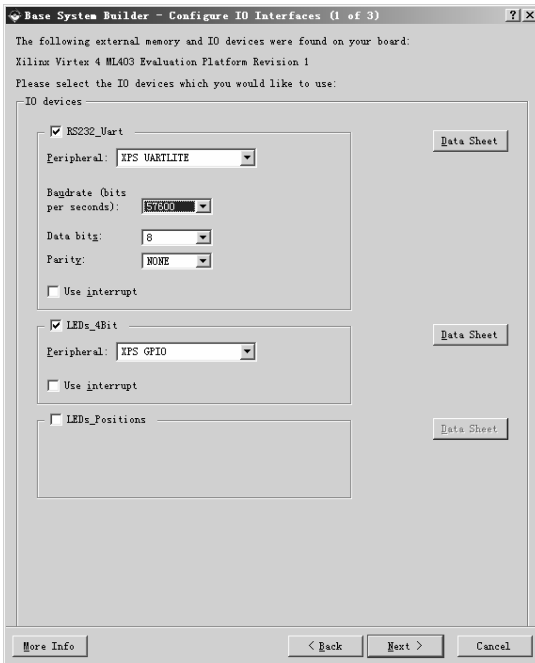
Figure 4: Configure I/O Interfaces-1
