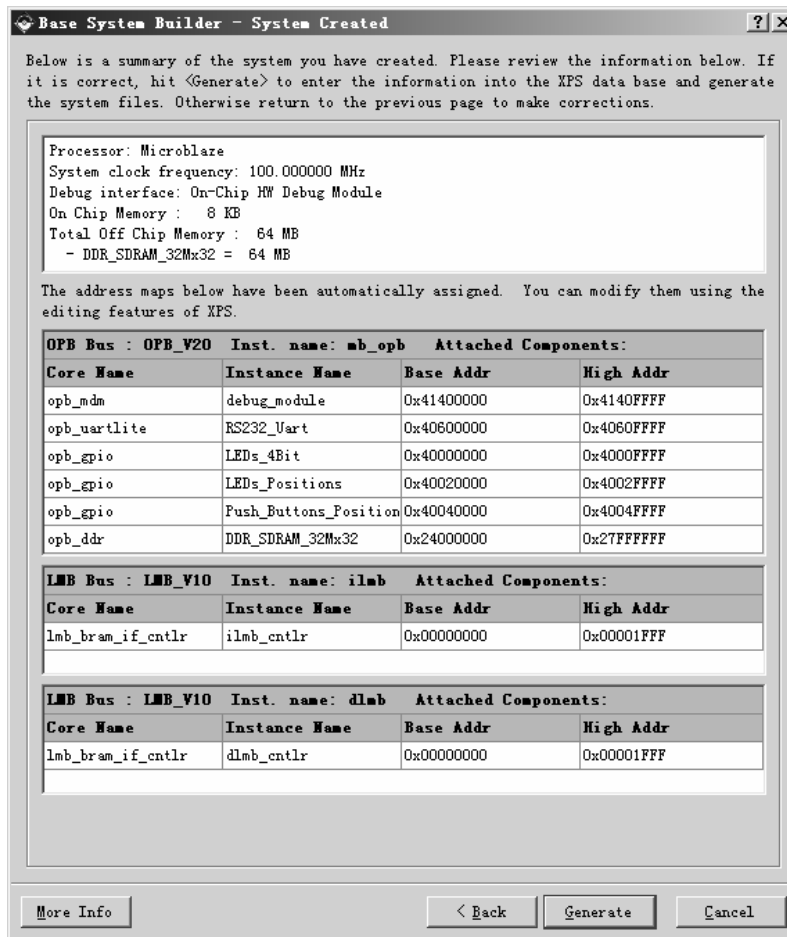
Figure 9: Completed Processor System
