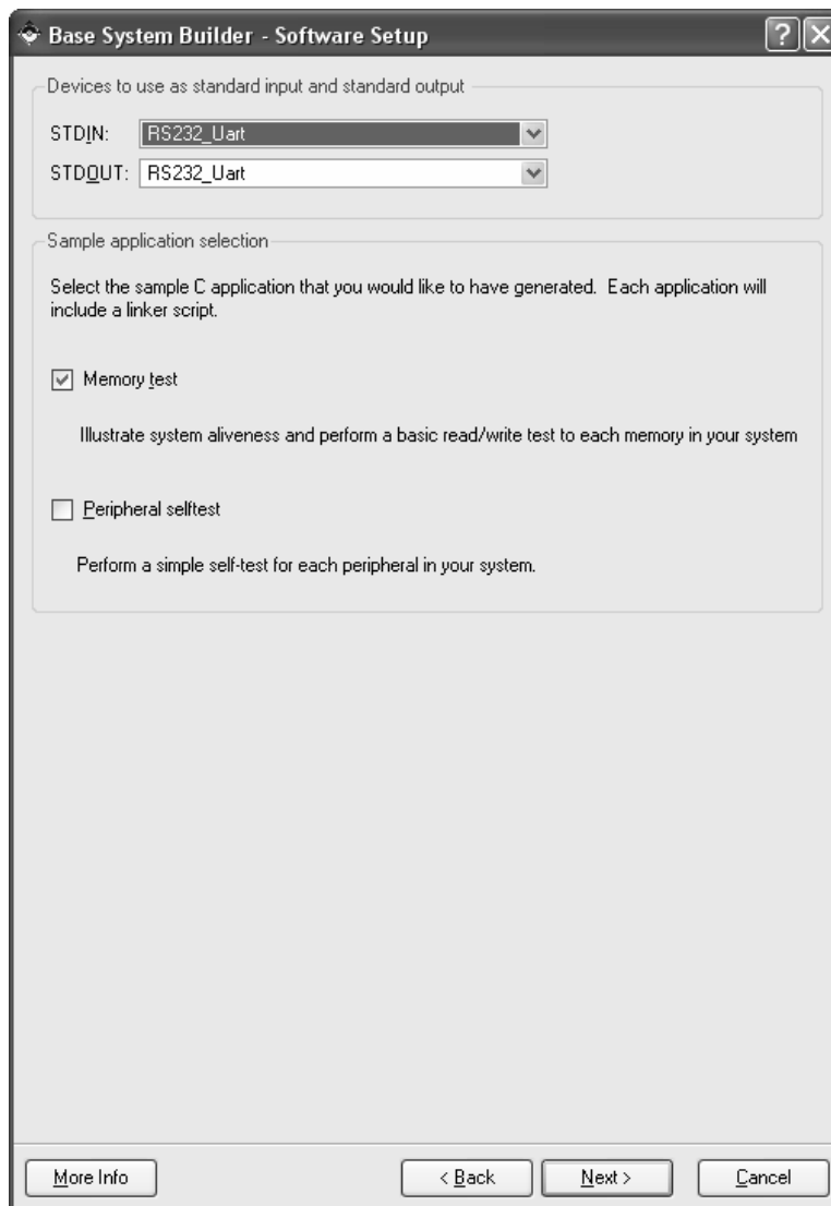
Figure 7: Software Setup
