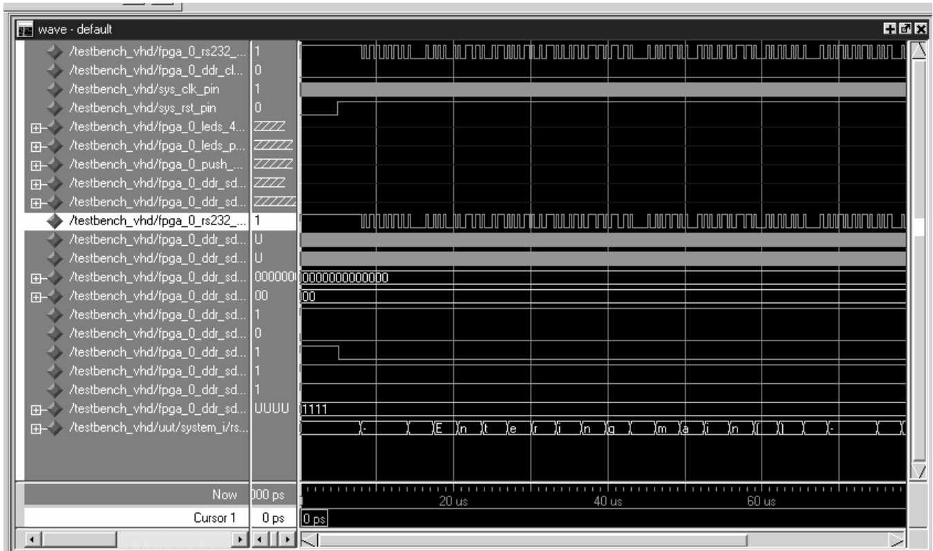
Figure37: Simulation results
