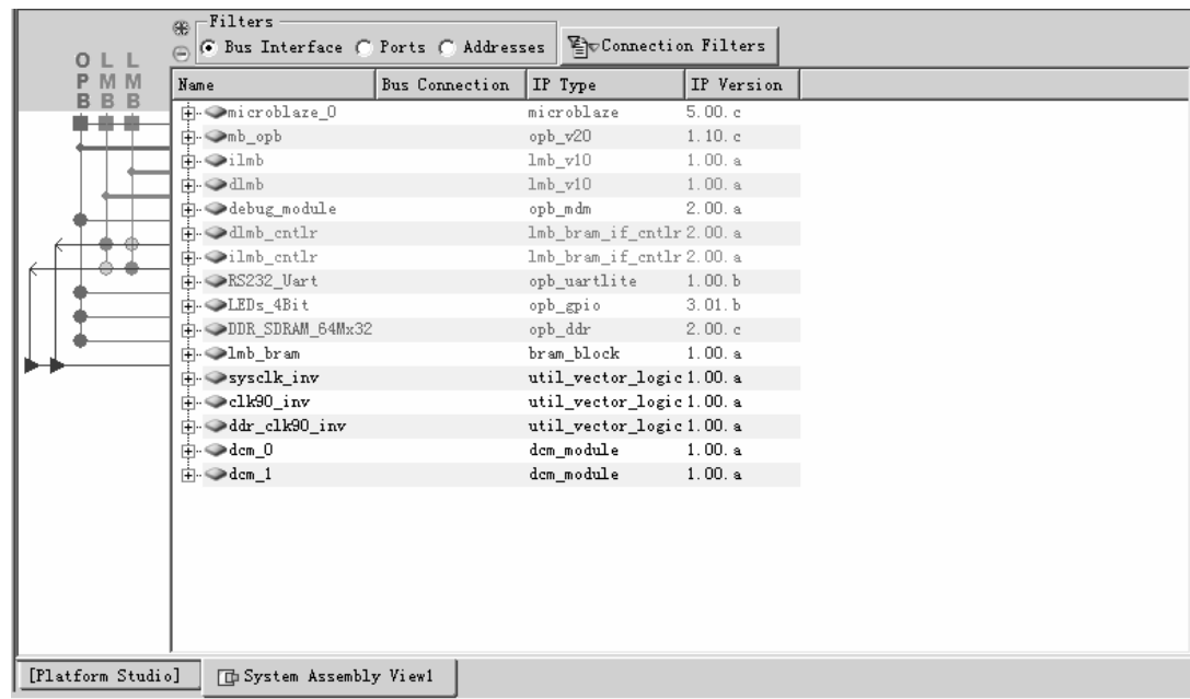
Figure 17: System Assembly View
