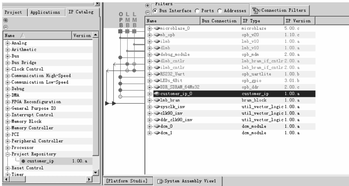
Figure 18: Inserting IP
