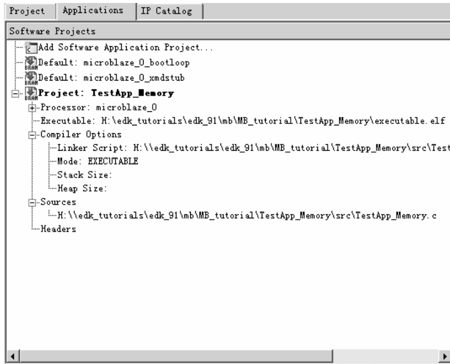
Figure 28: Applications Tab
