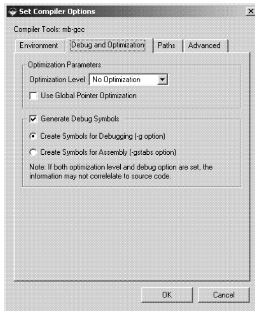
Figure 33: Compiler Options
