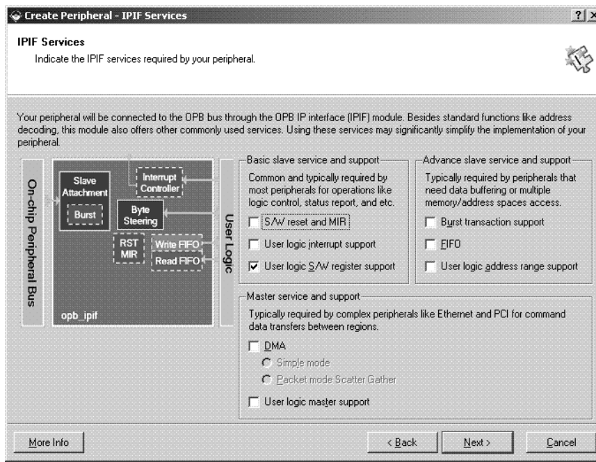
Figure 14: Create Peripheral - IPIF Services
