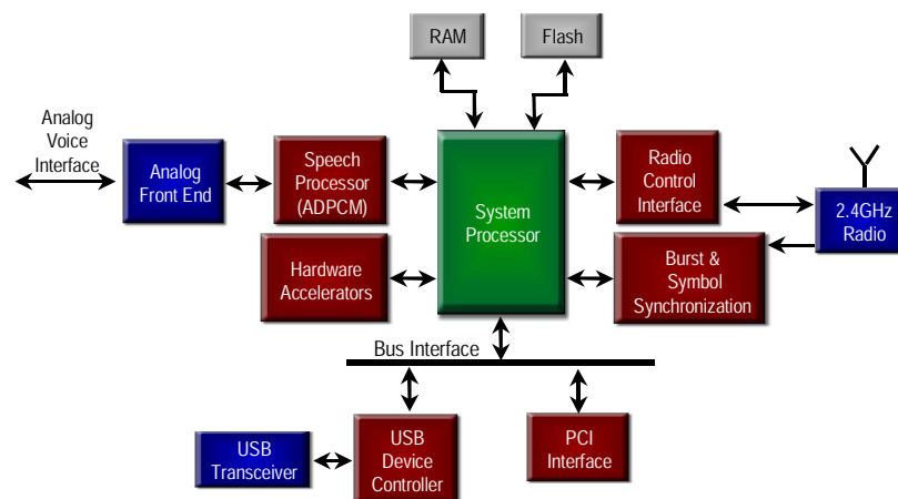
Figure 2: HomeRF Module
