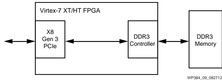
Figure 1: Interfacing DDR3 Memory to Virtex-7 XT/HT FPGAs
