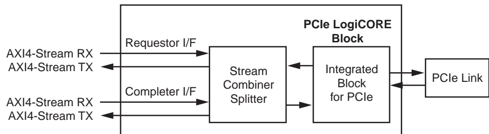
Figure 3: Enhanced AXI4-Stream Interface
