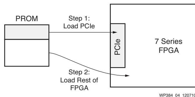
Figure 5: Tandem PROM Method
