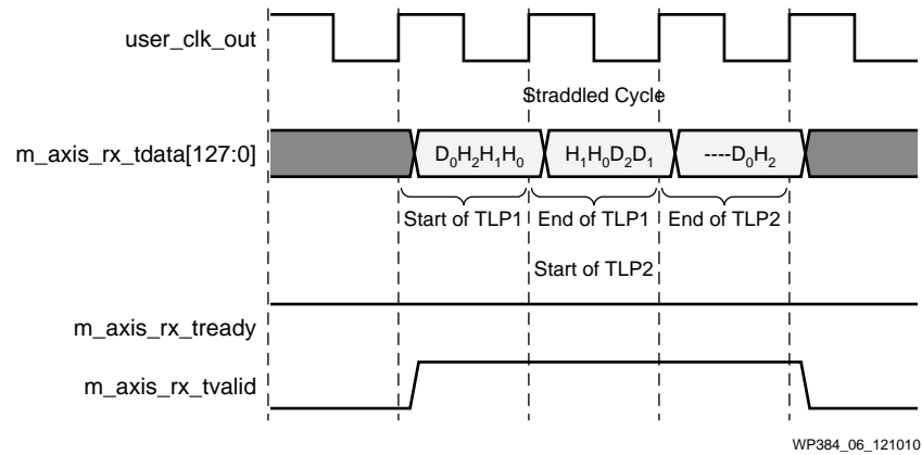
Figure 7: 7 Series Straddled Cycle
