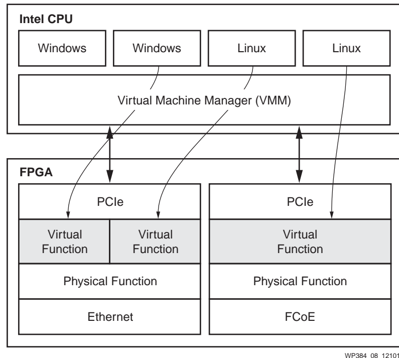
Figure 9: SR-IOV Virtual Configuration Space
