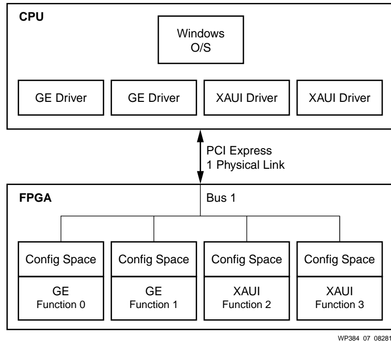
Figure 8: Multiple Function Devices
