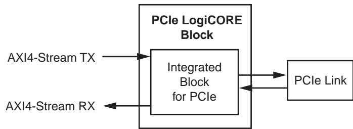
Figure 2: Basic AXI4-Stream Interface
