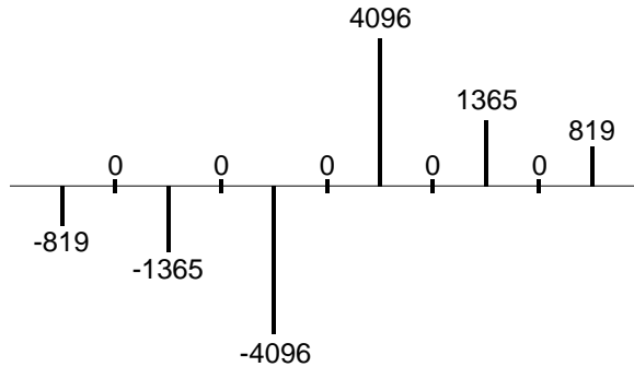
Figure 3-22: Hilbert Transformer Impulse Response
