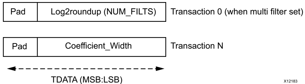
Figure 3-5: tdata Format
