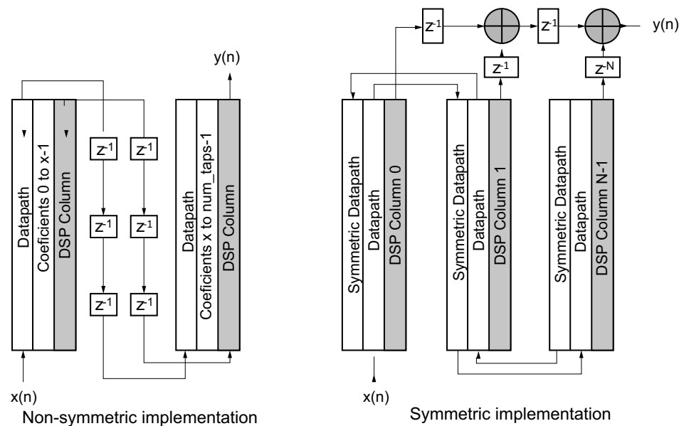
Figure 3-61: Multi-Column Implementations
