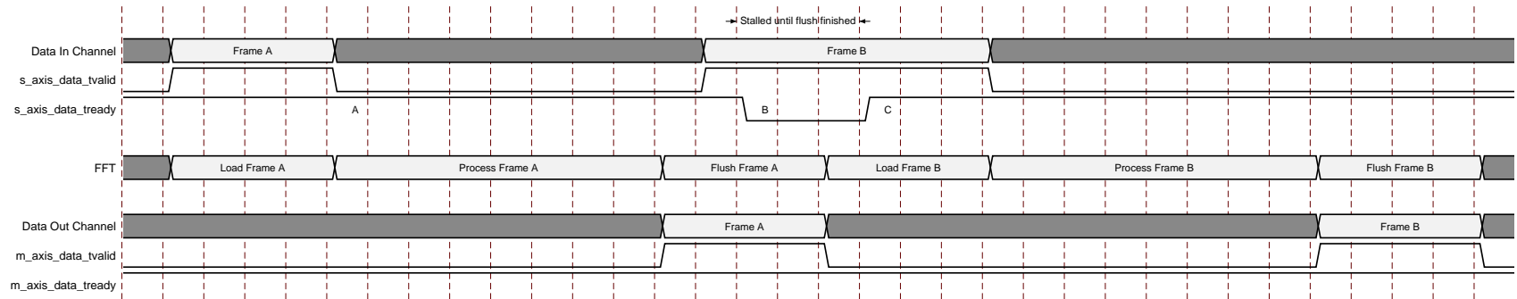
Figure 3-46: Transform Timing for Entire Frames In Burst I/O Mode with Bit-Reversed Outputs (Core Flushes Frame)
