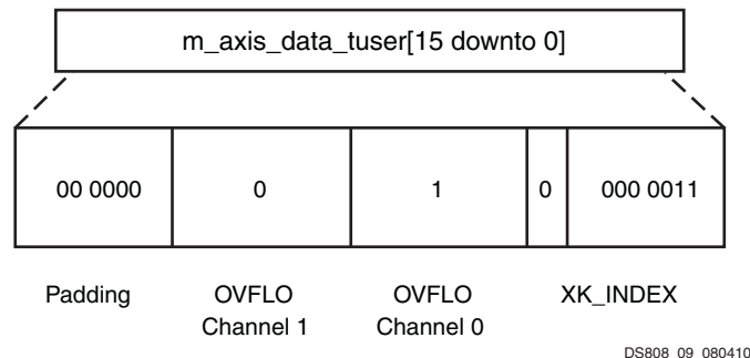
Figure 3-9: Data Output Channel TUSER Example 1
