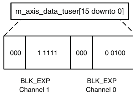
Figure 3-10: Data Output Channel TUSER Example 2
