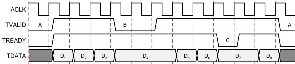
Figure 3-40: AXI Transfers and Terminology
