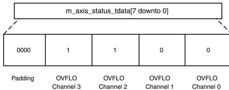
Figure 3-12: Status Channel TDATA Example 1
