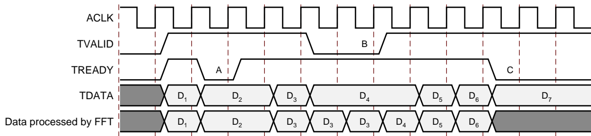
Figure 3-41: Incorrect Transfer in Realtime mode
