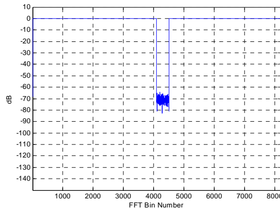
Figure 3-32: 8192-point Transform
