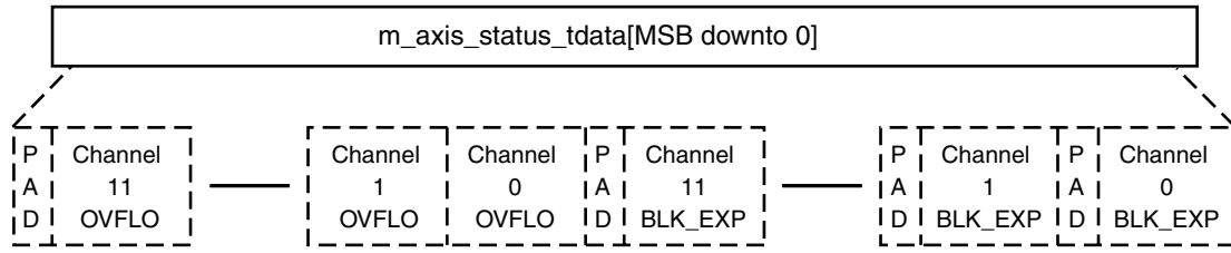
Figure 3-11: Status channel TDATA (m_axis_status_tdata) Format
