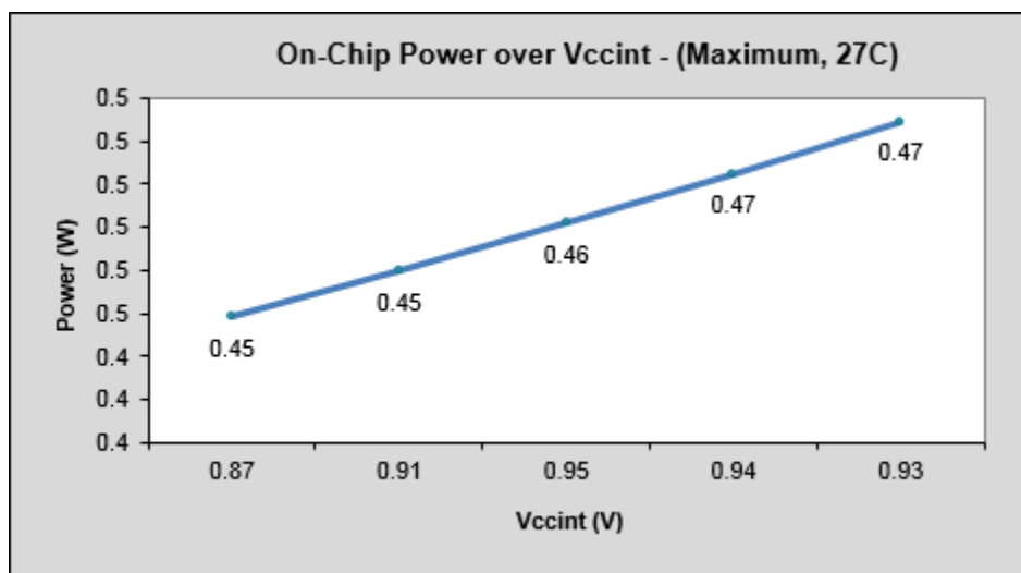
Figure 52: Graph Displaying On-Chip Power Over Vccint
