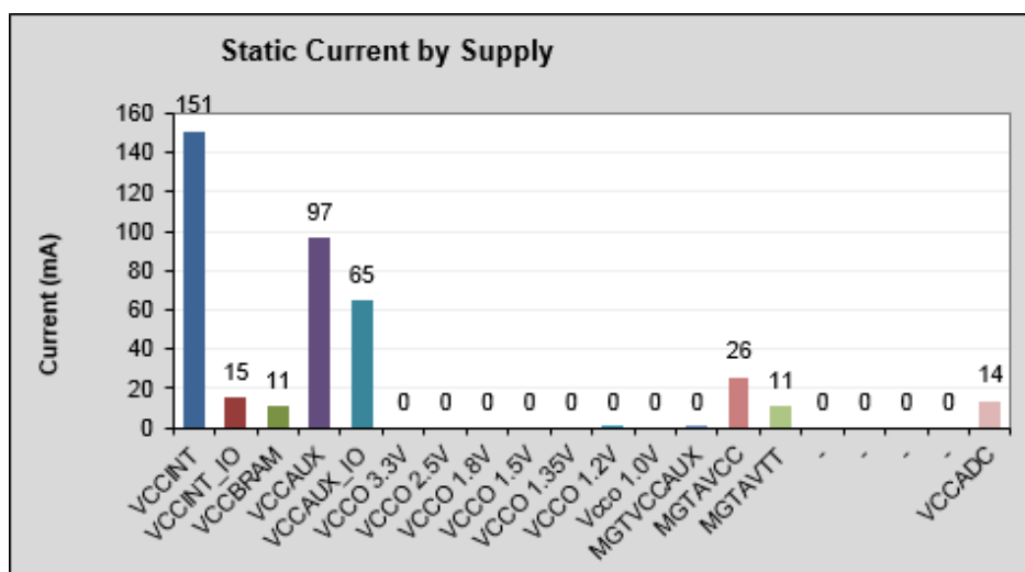
Figure 53: Graph Displaying the Static Current by Supply
