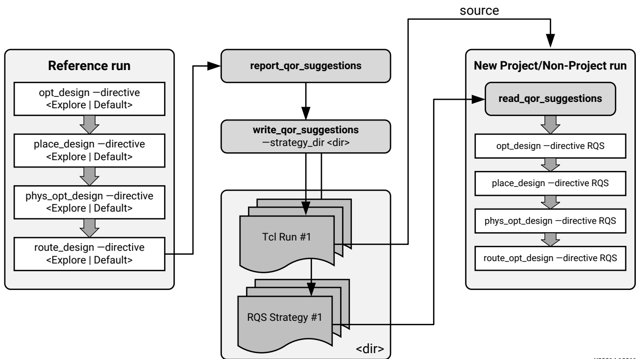
Figure 225: Strategy Suggestion Flow
