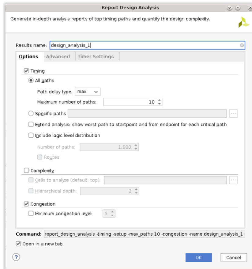
Figure 169: Report Design Analysis Dialog Box
