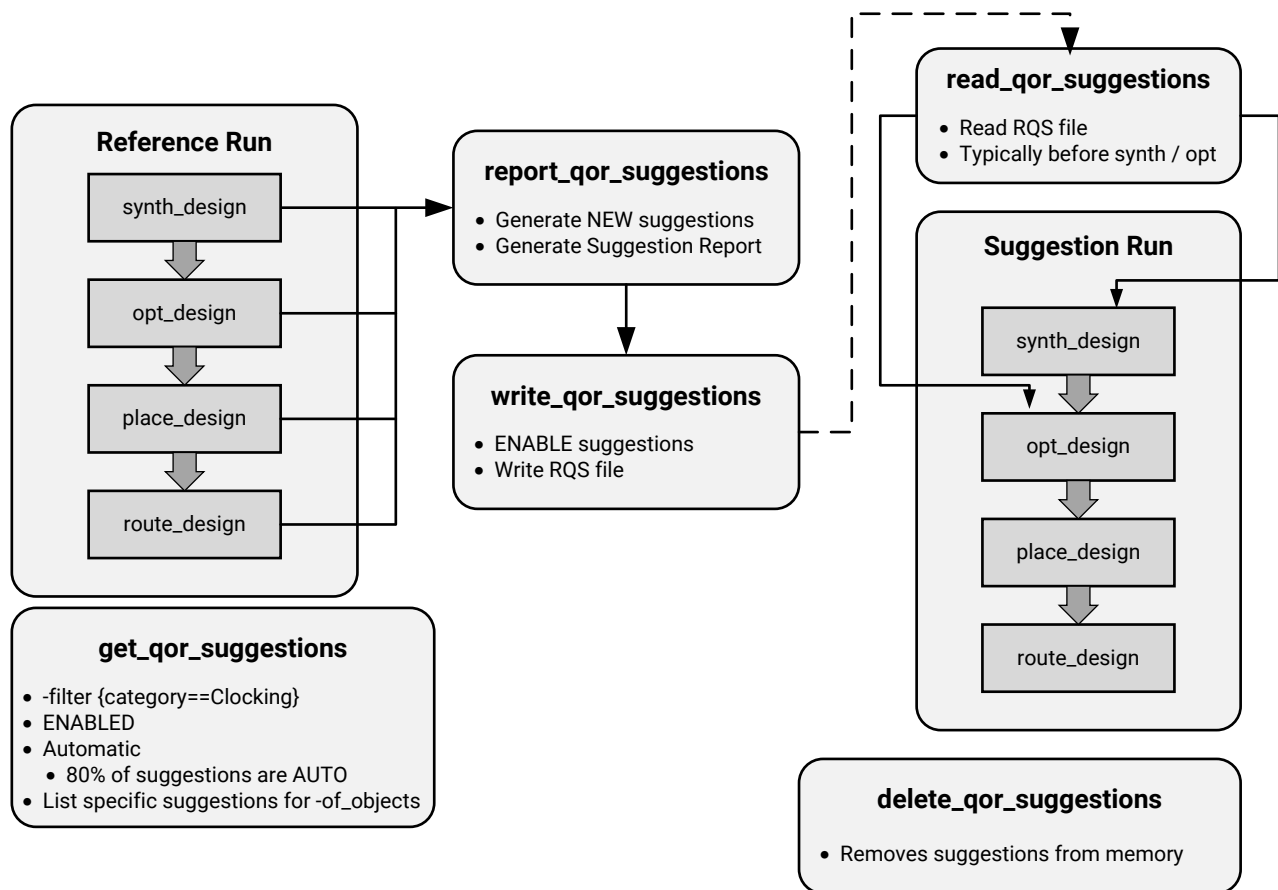
Figure 220: Suggestion Flow
