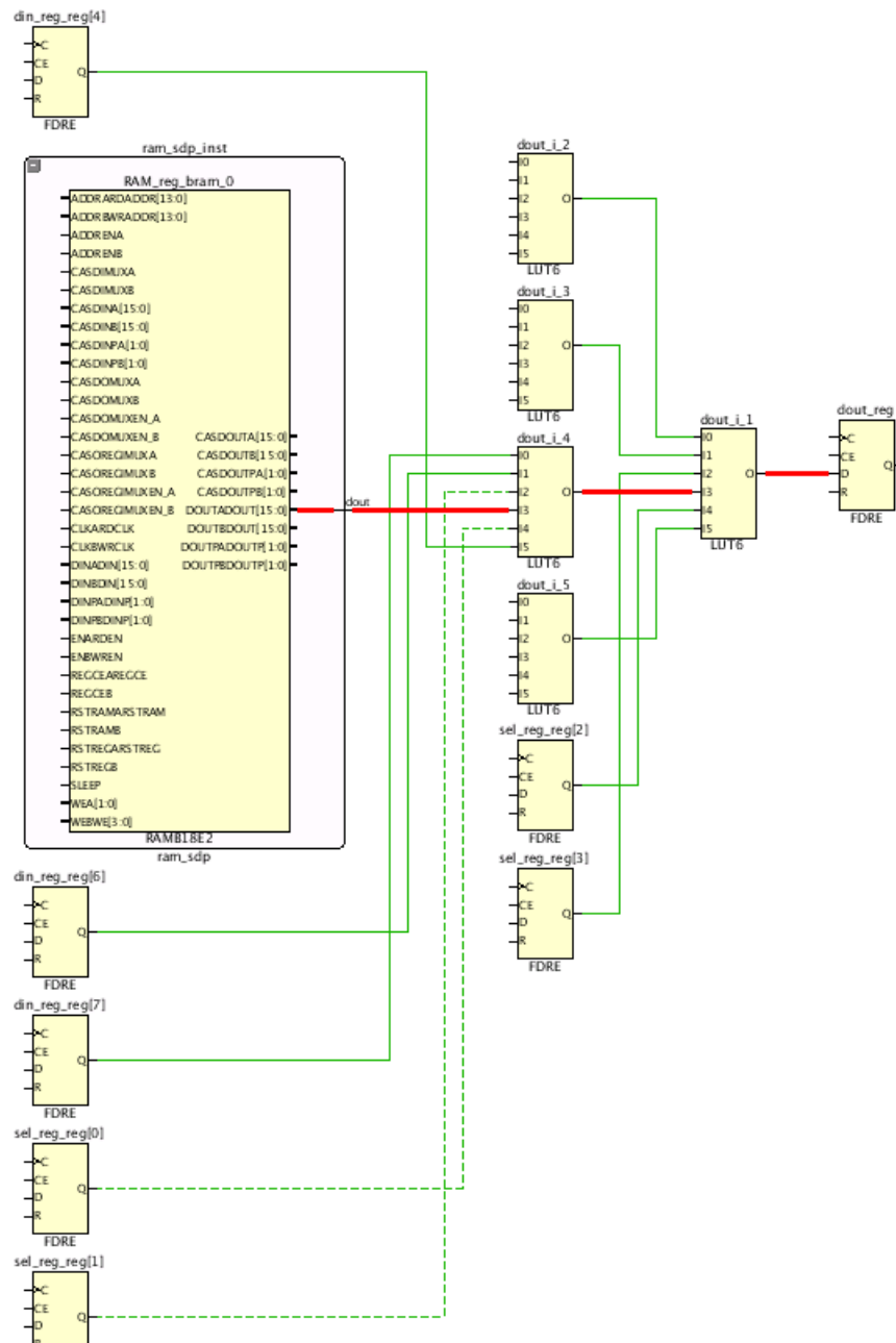
Figure 210: Critical RAMB-LUT-FF Path
