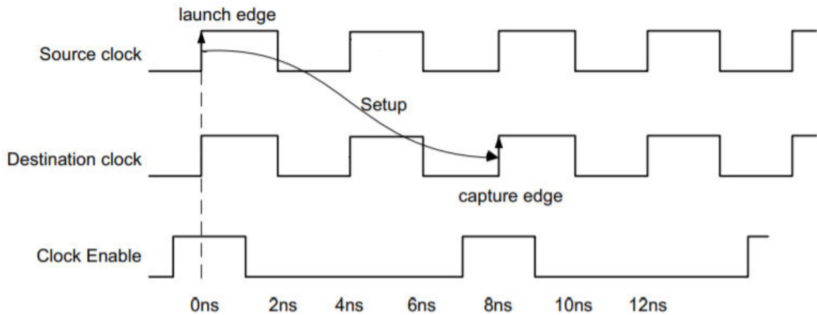
Figure 255: Timing Diagram
