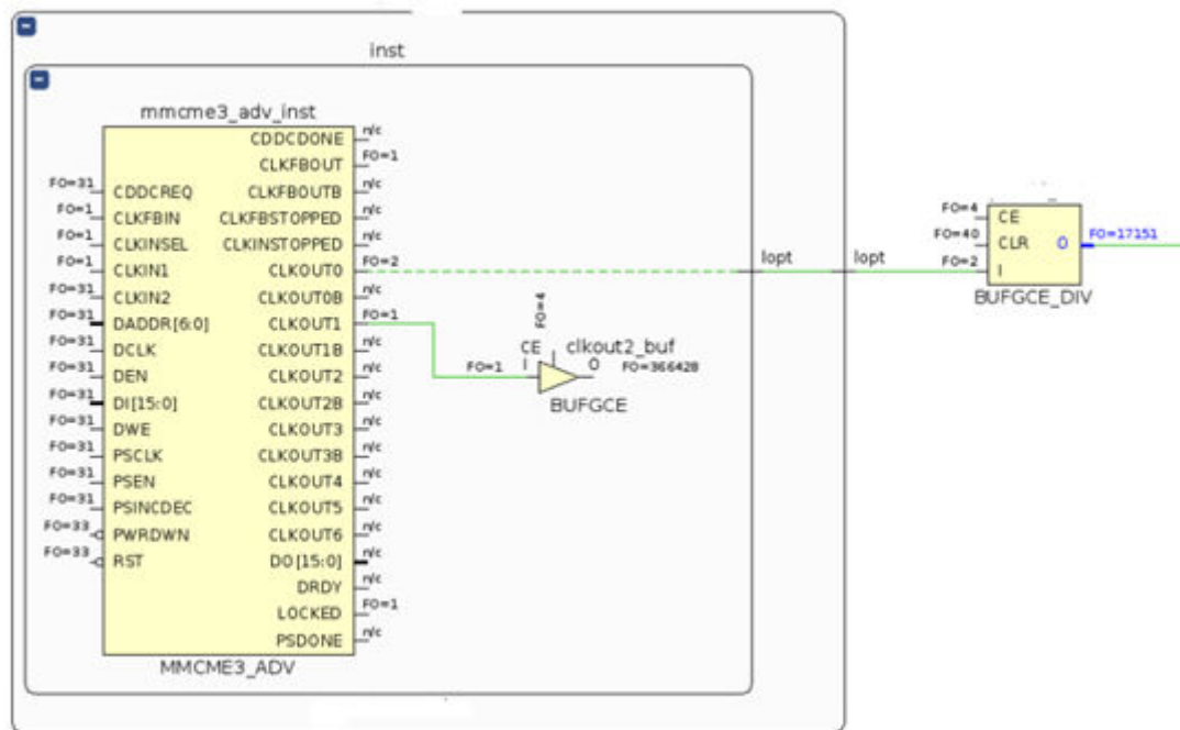
Figure 256: False Path, Asynchronous Clock Group, or Max Delay Datapath Only Constraint between Synchronous Clocks
