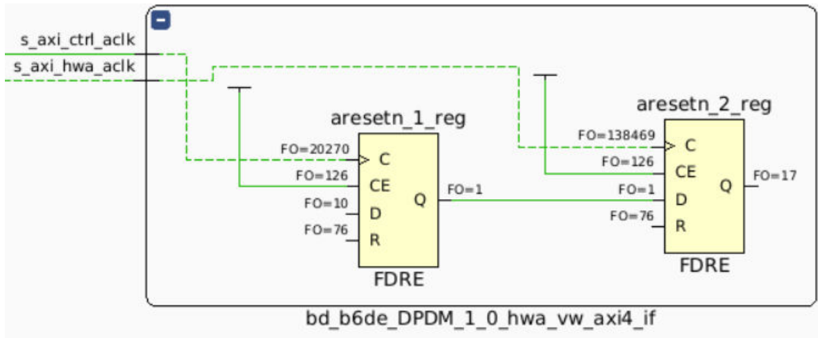
Figure 253: Multicycle Path with Tied CE Pins Example
