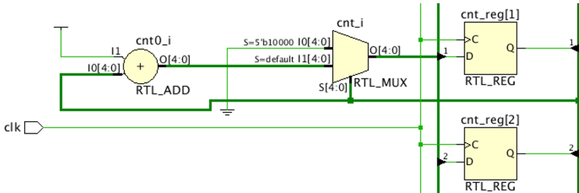
Figure 193: cnt Counter in the Elaborated View after RTL Improvement
