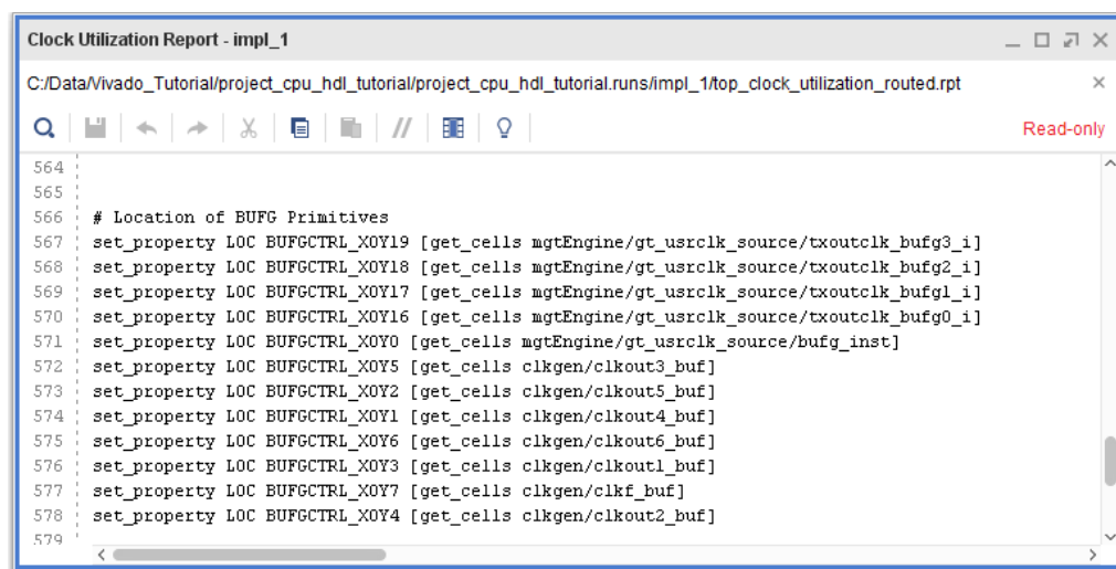
Figure 227: Clock Locations
