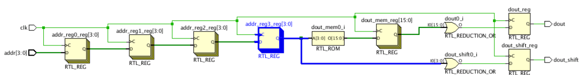
Figure 205: Elaborated View of RTL Code Snippet
