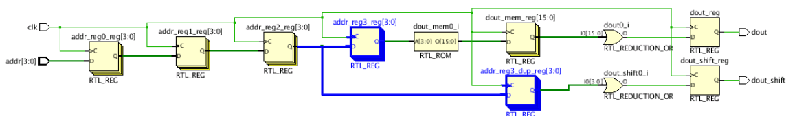
Figure 207: Elaborated View of the Replicated Address Register
