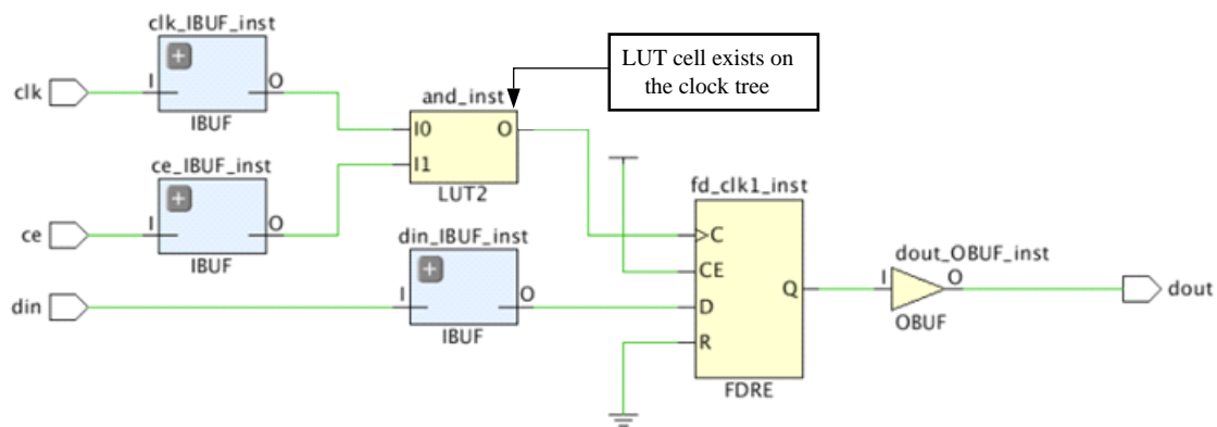
Figure 252: LUT on the Clock Tree
