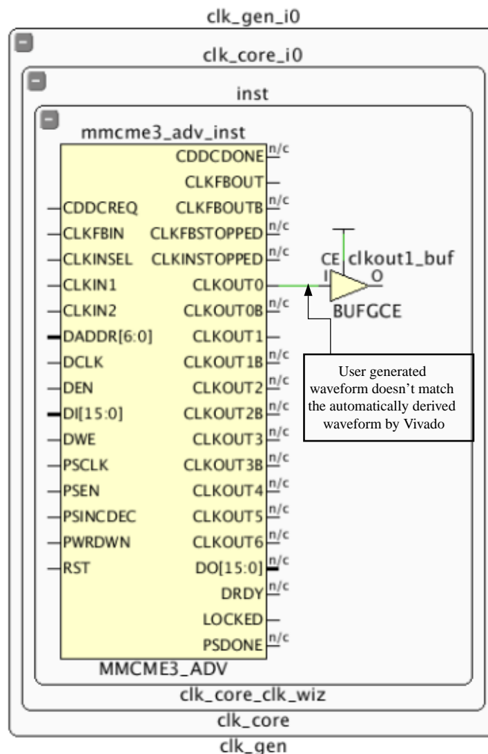
Figure 244: Invalid Clock Waveform on Clock Modifying Block
