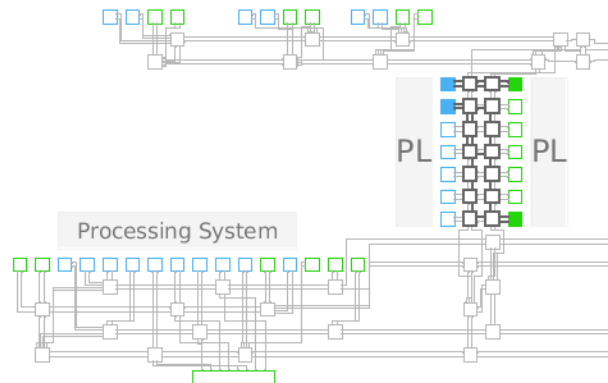
Figure 242: NoC Solution with manual NSU assignment
