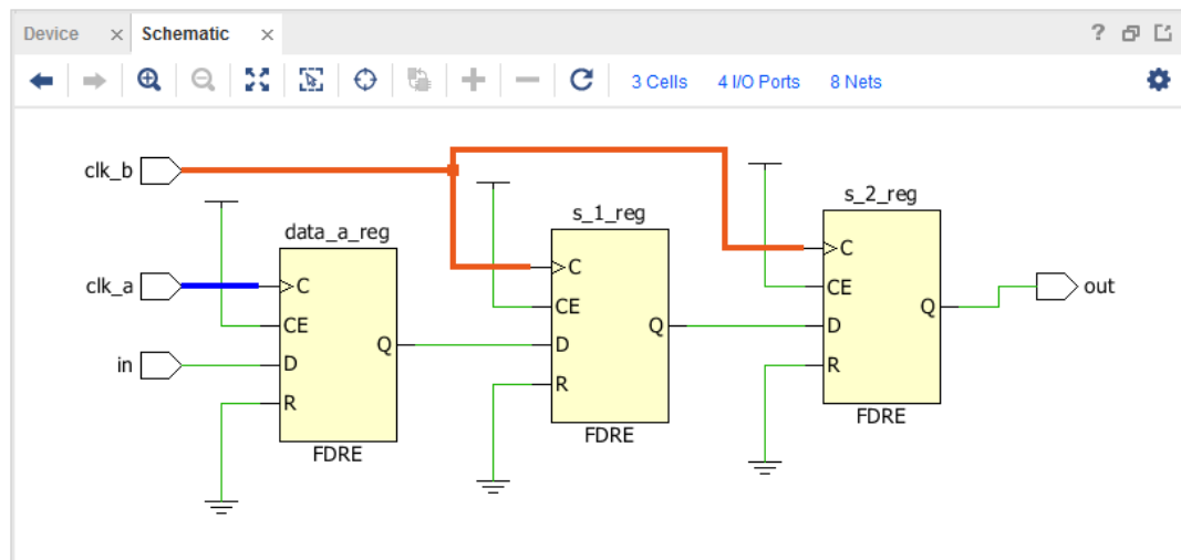
Figure 145: Simplified Topology of a Single-Bit Synchronizer
