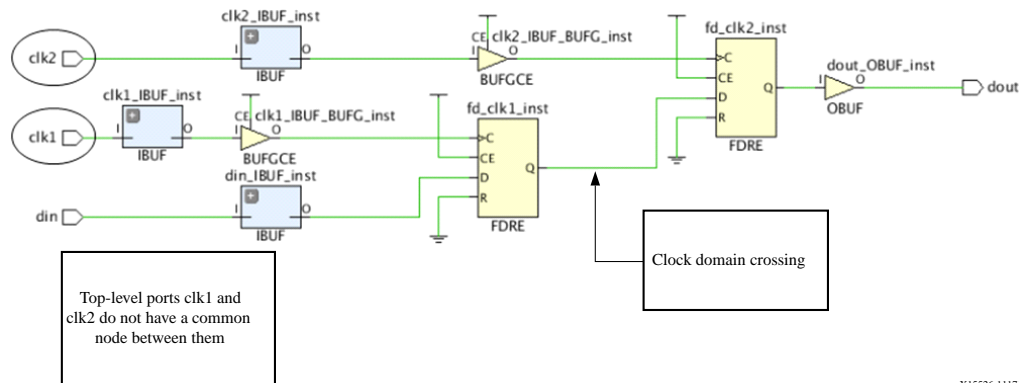
Figure 249: No Common Node Between Related Clocks
