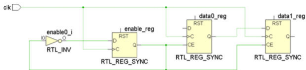
Figure 254: Flop-to-Flop Path
