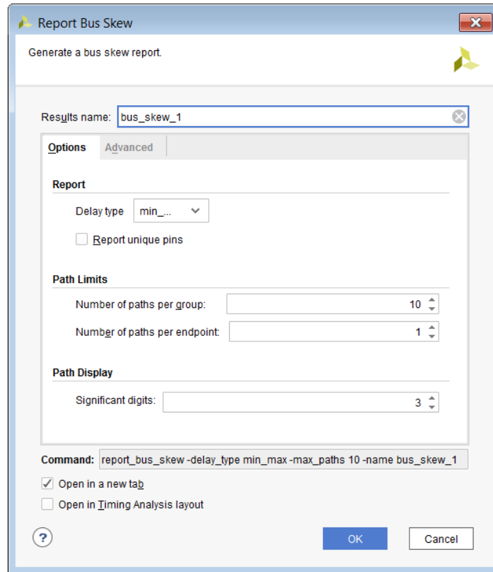
Figure 106: Report Bus Skew Dialog Box: Options Tab
