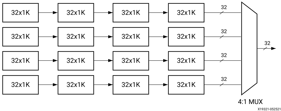
Figure 195: Generated Structure for 32 \times 16K Memory Configuration using RAM_DECOMP and CASCADE_HEIGHT Attributes
