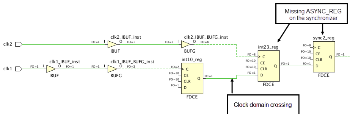
Figure 251: Missing Property on Synchronizer
