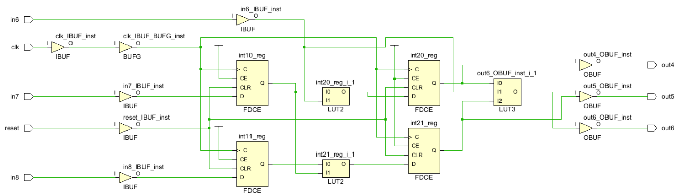
Figure 121: Fully Constrained Design for Timing Exception Example
