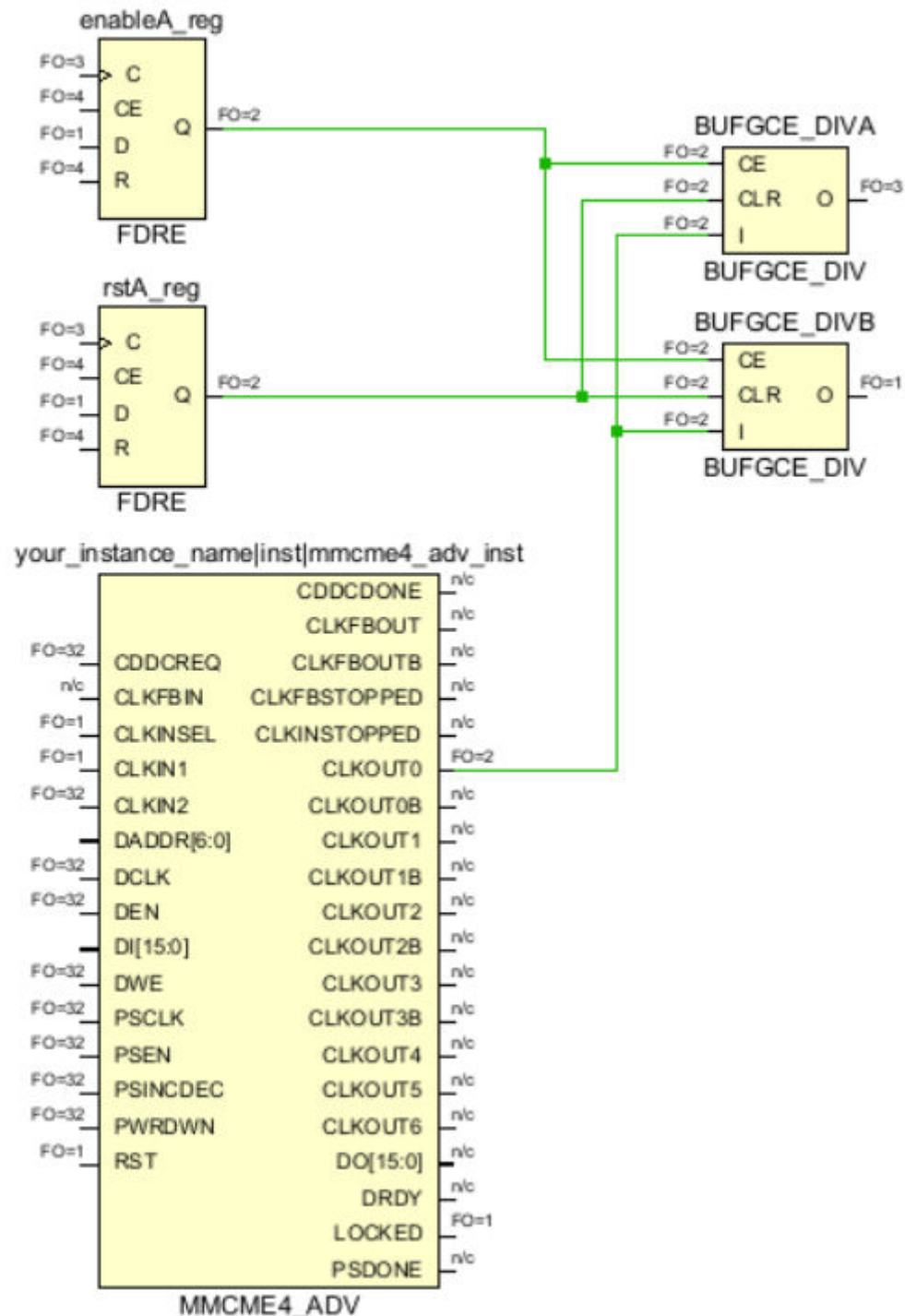
Figure 257: Correct Implementation of BUFGCE_DIV Buffers
