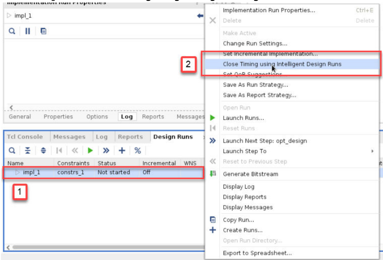
Figure 216: Close Timing Using Intelligent Design Runs Command
