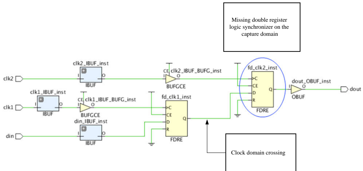
Figure 250: Missing Synchronizer
