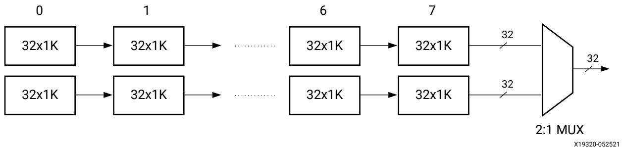
Figure 197: Generated Structure for 32 \times 16K Memory Configuration using RAM_DECOMP Attribute
