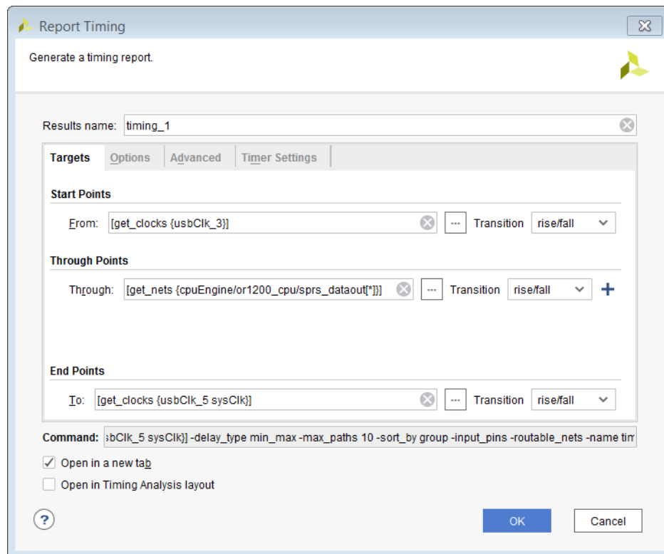
Figure 85: Report Timing Dialog Box: Targets Tab
