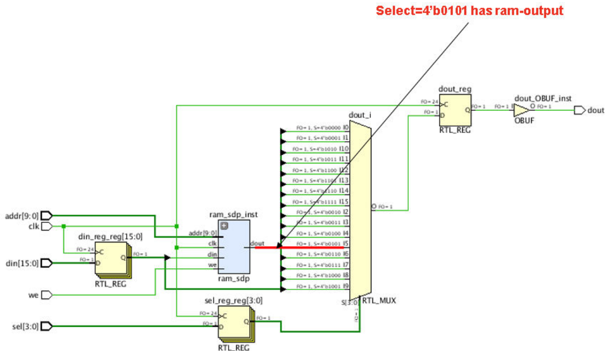
Figure 209: 16x1 Multiplexer Connected to Block RAM Outputs
