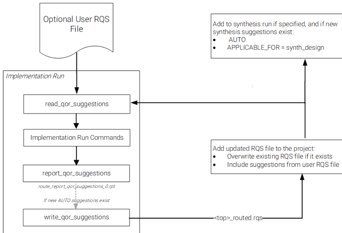
Figure 223: Implementation Flow with Automatic QoR Suggestions
