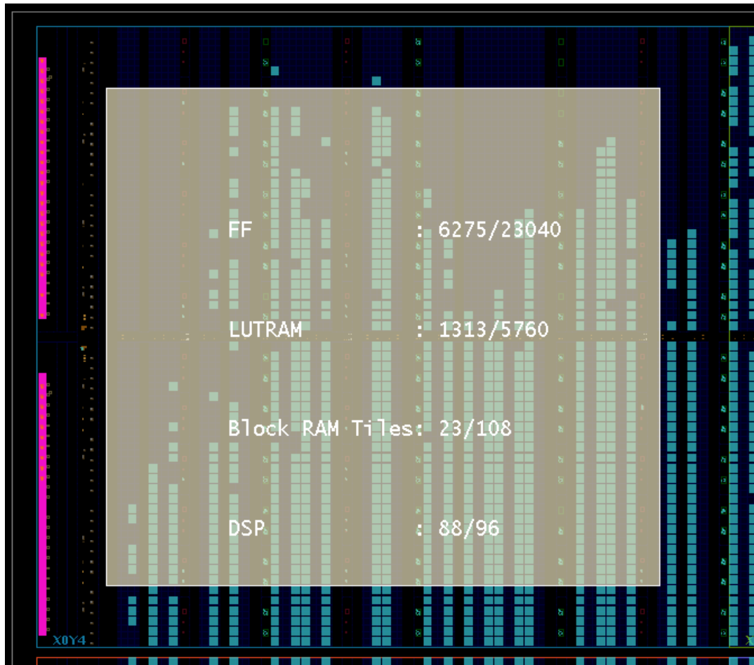
Figure 69: Report Clock Utilization - Clock Region Resource Utilization Metrics in the Device Window
