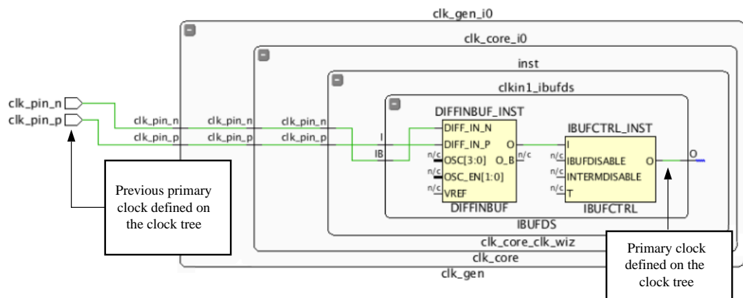
Figure 247: Invalid Primary Clock Redefinition on a Clock Tree
