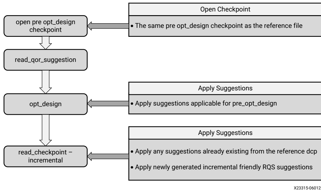
Figure 224: Incremental Flow
