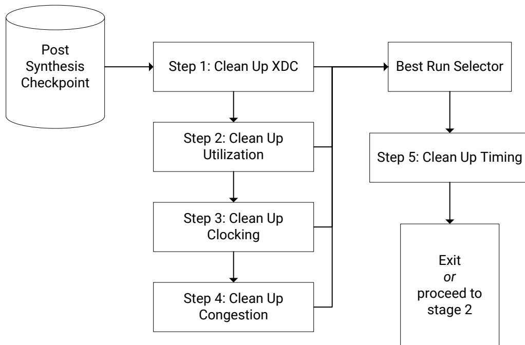
Figure 214: Design Optimization Steps
