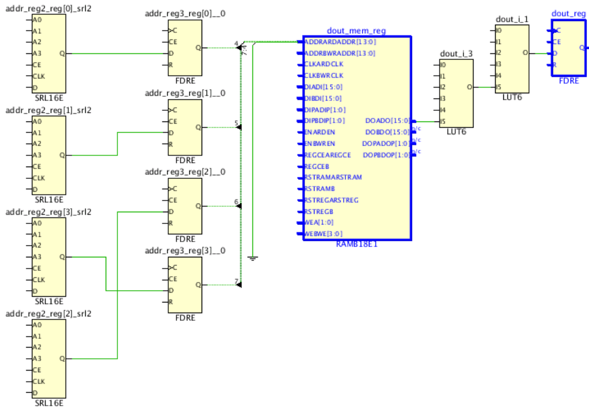
Figure 204: Critical Path from RAMB Without Output Register Enabled
