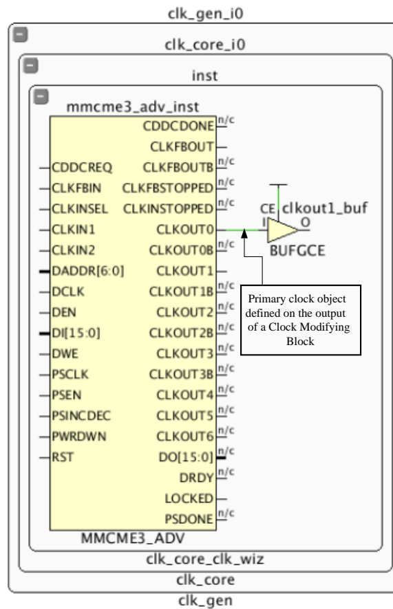
Figure 246: Invalid Primary Clock on Clock Modifying Block
