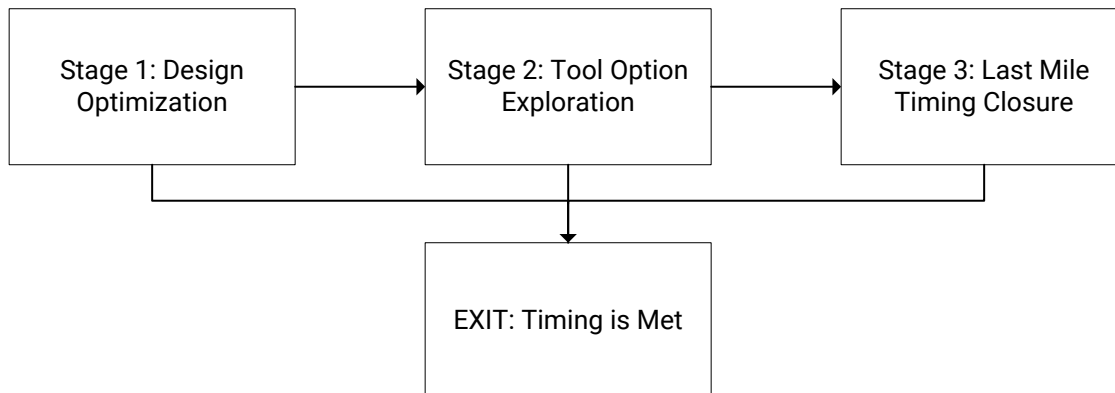
Figure 213: IDR Overview
