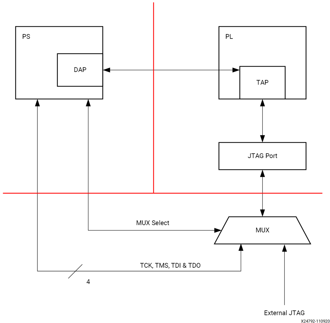
Figure 2: MUX Usage
