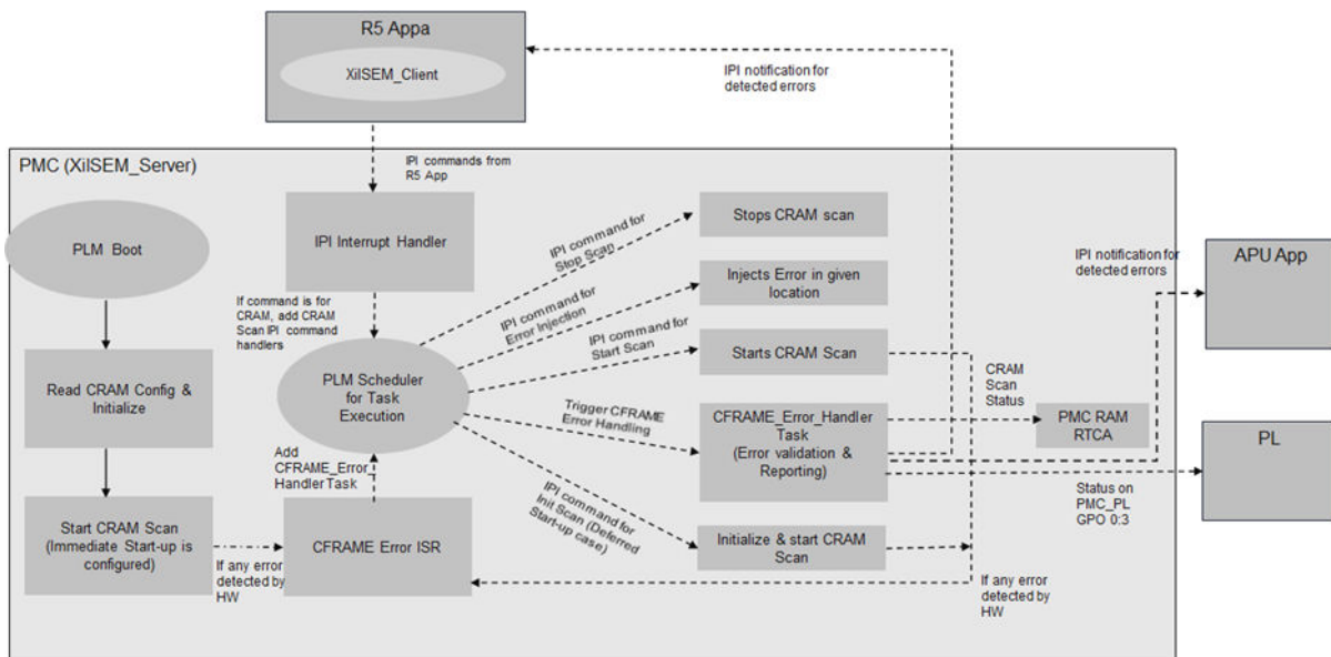
Figure 11: Software Flow for CFRAME Scan
