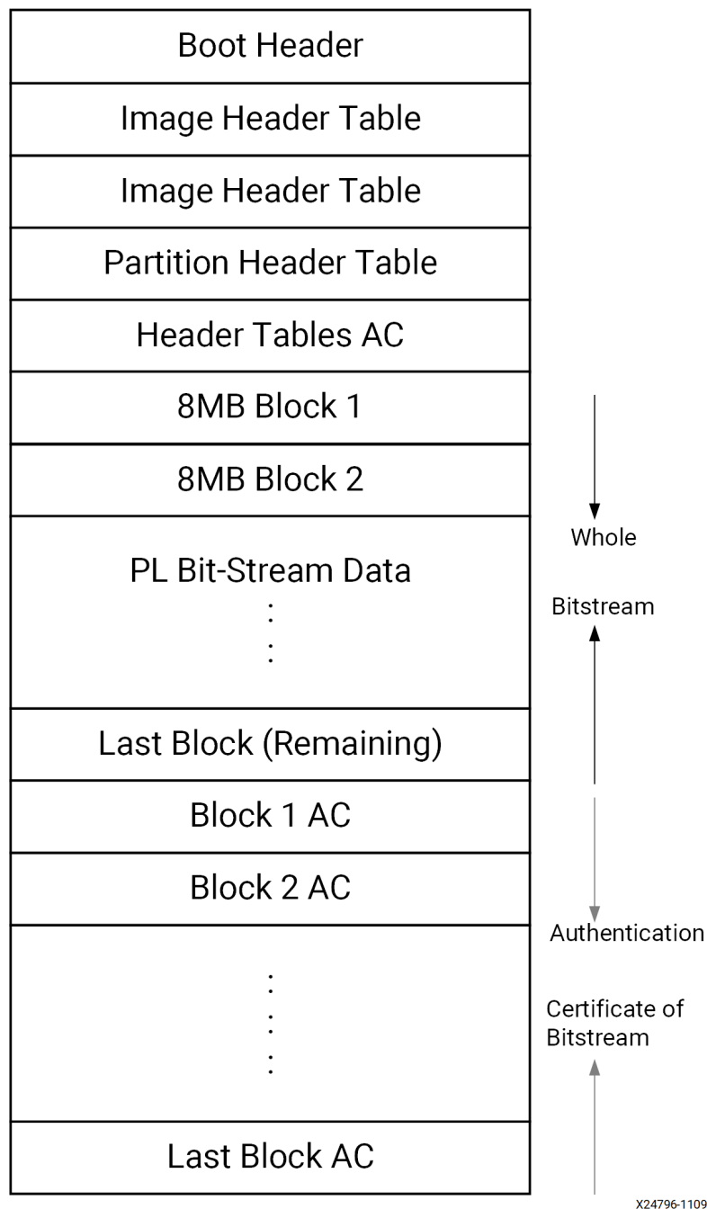
Figure 7: Bitstream Blocks
