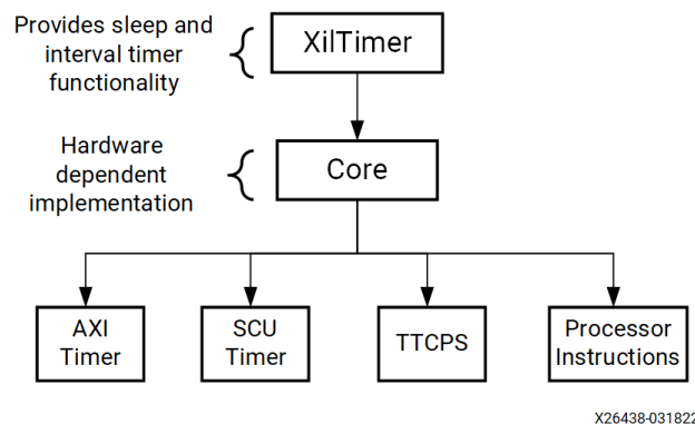
Figure 13: XilTimer Library
