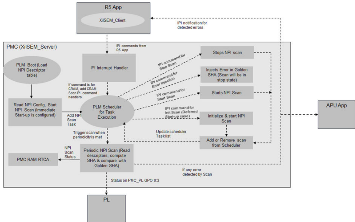
Figure 12: Software Flow for NPI Scan
