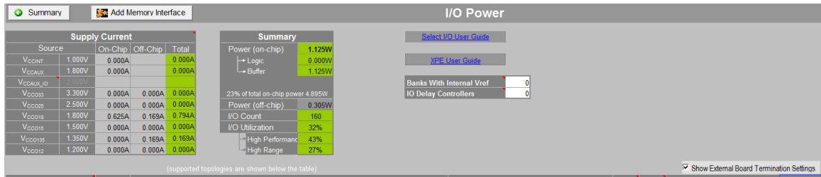
Figure 18: I/O Sheet - Top Section (7 Series Devices)
