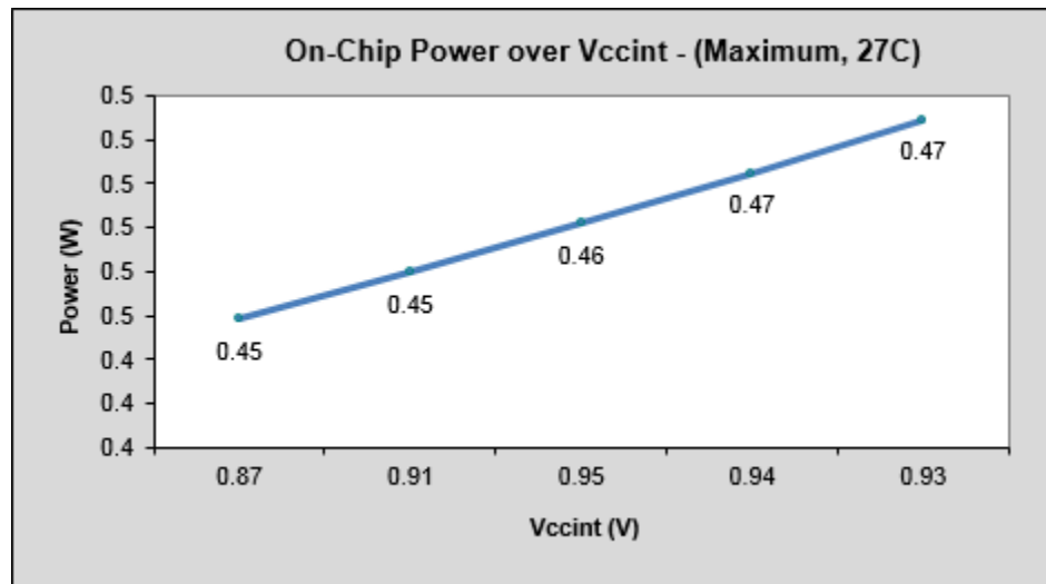
Figure 52: Graph Displaying On-Chip Power Over Vccint
