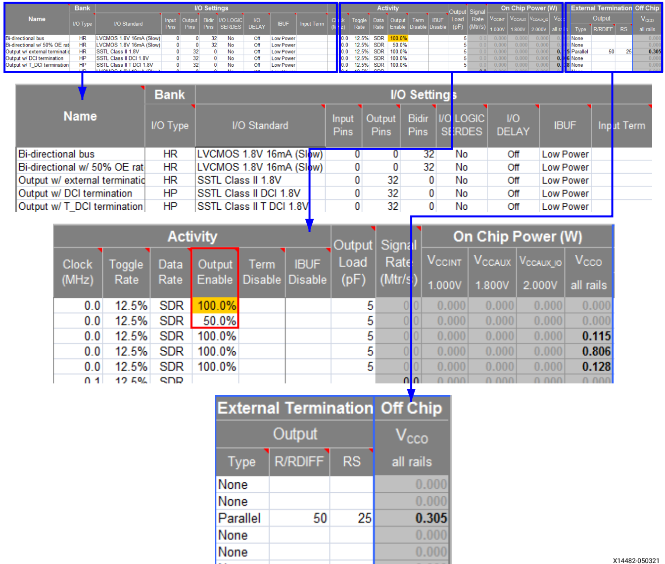
Figure 19: I/O Sheet - Effect of Output Enable Rate on Power Estimates for Inputs, Outputs, and Bidirectional I/Os (7 Series Devices)
