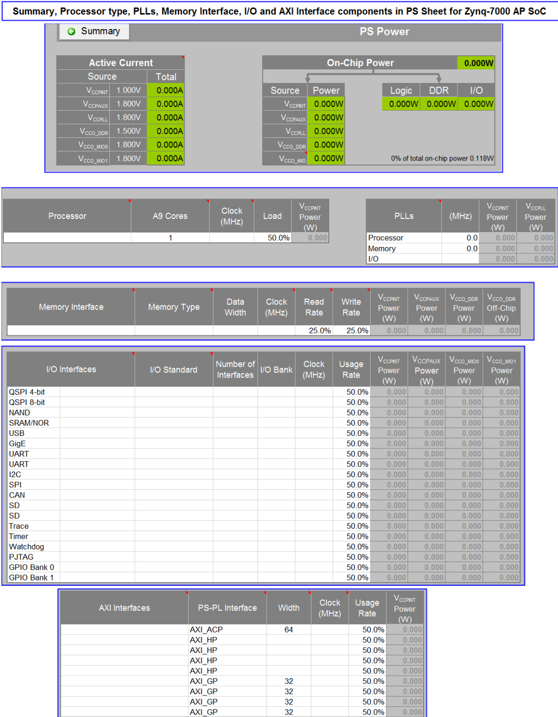
Figure 30: PS Sheet for Zynq-7000 SoC
