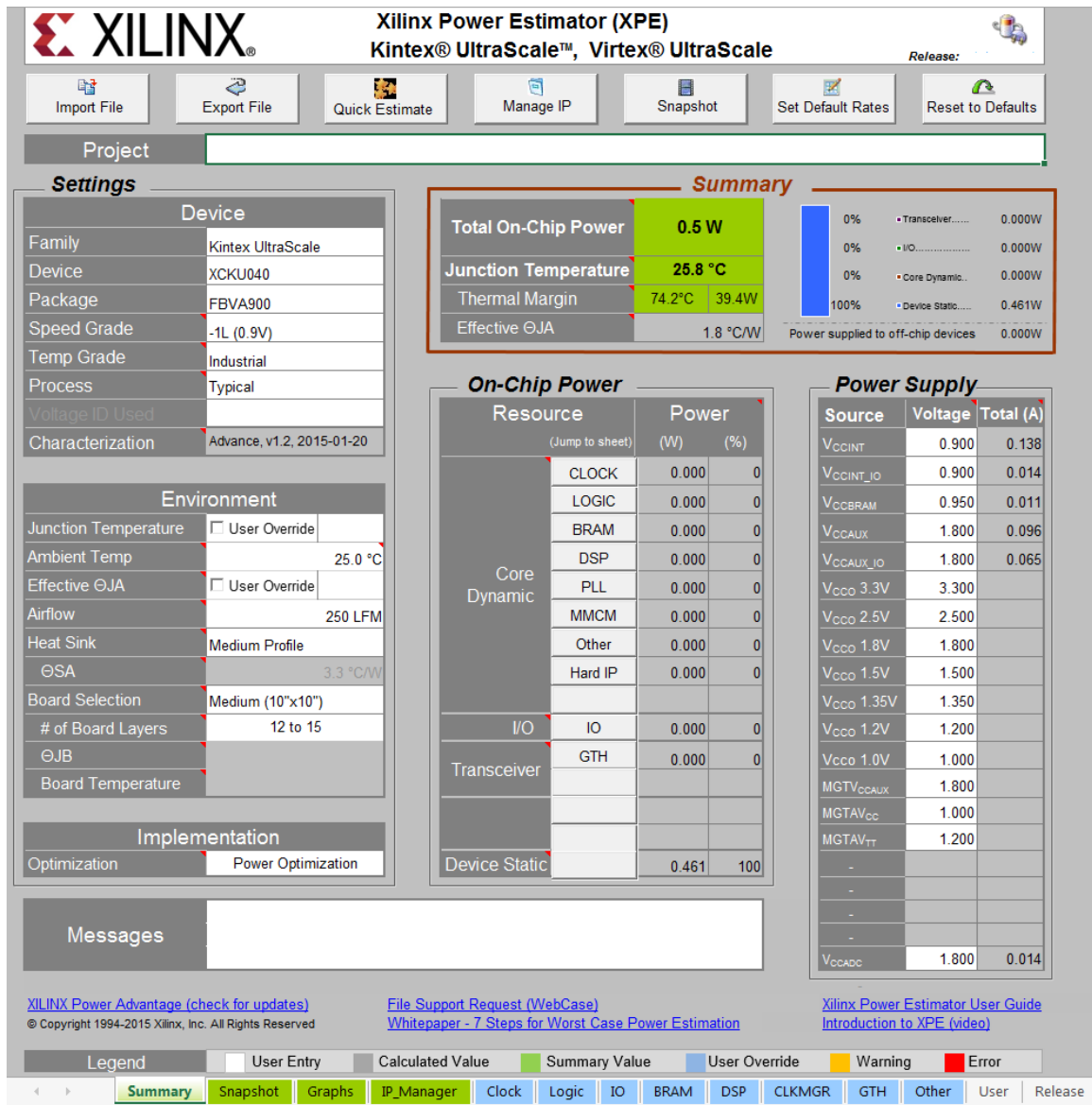
Figure 1: Xilinx Power Estimator Spreadsheet
