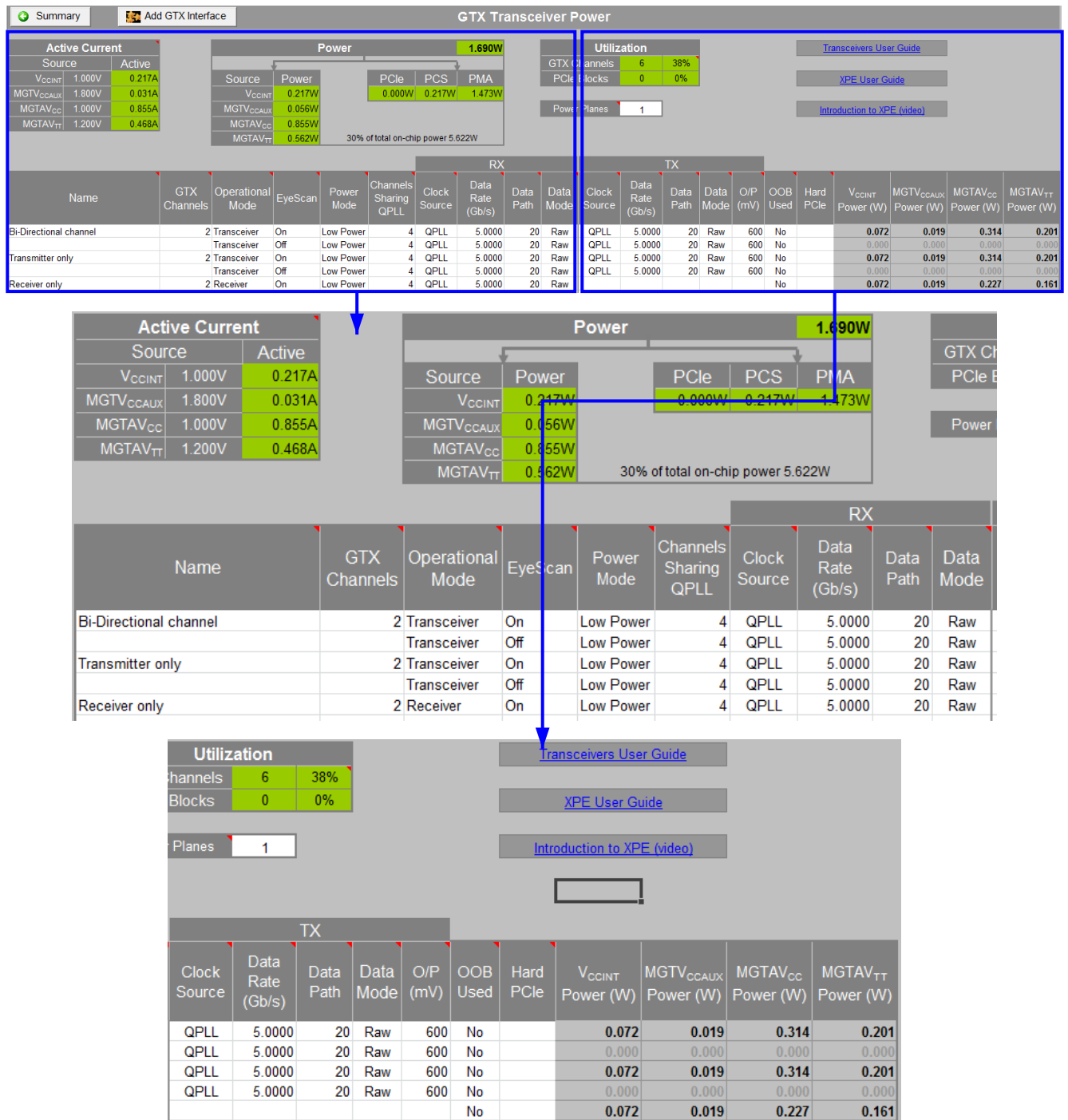
Figure 24: GT Power Sheet (Kintex-7 Devices) Illustrating Data Rate and Power Estimates
