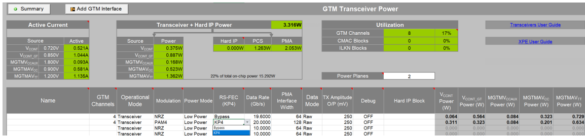
Figure 26: GTM Transceiver Power
