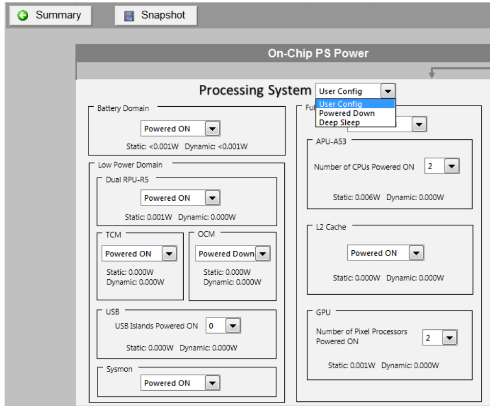
Figure 32: PS Sheet for Zynq UltraScale+ MPSoC Displaying Sources and Power Supply
