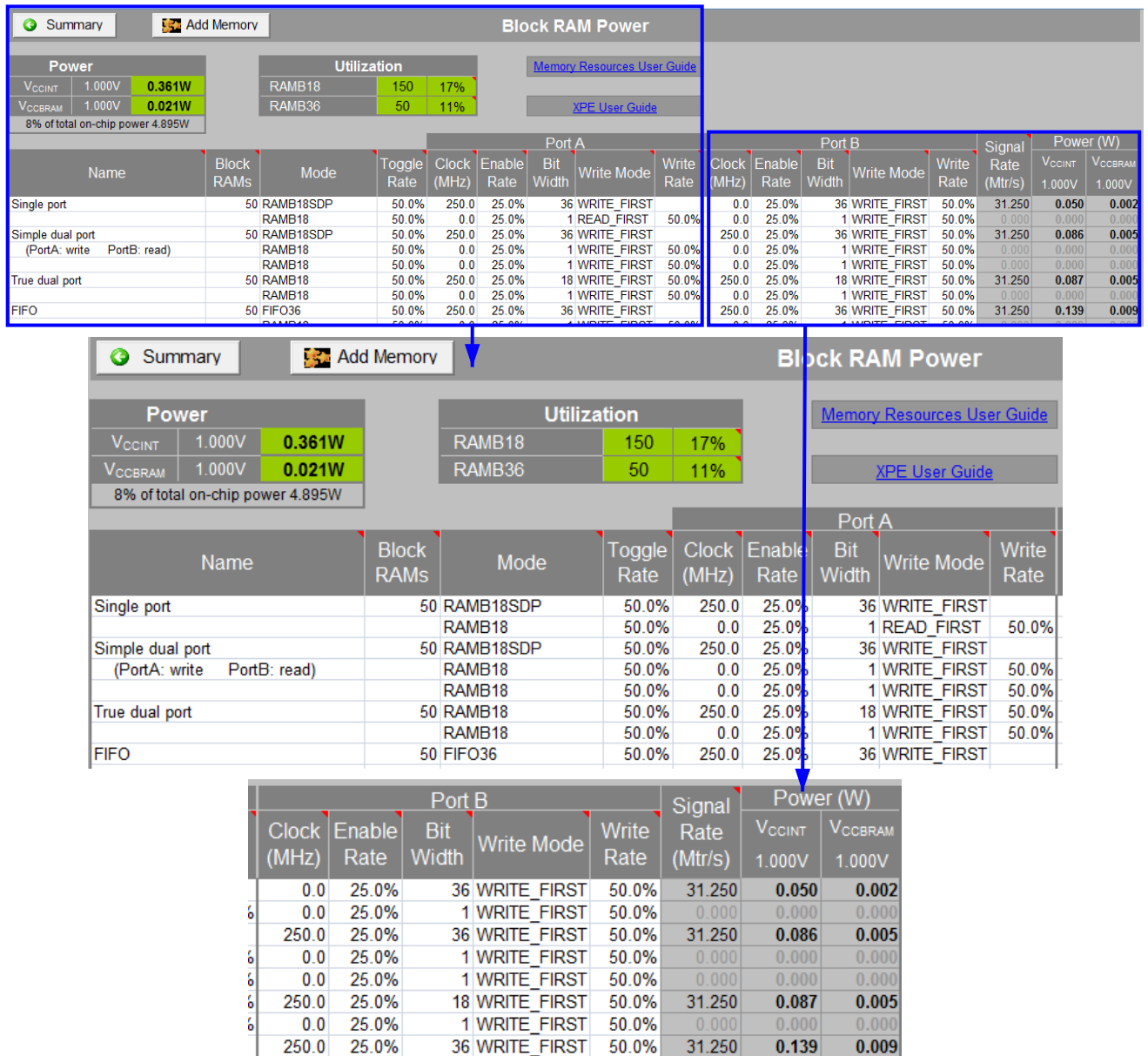
Figure 21: Block RAM Sheet - Effect of Block RAM Configuration Modes and Bit Widths on Power Estimates (7 Series Devices)
