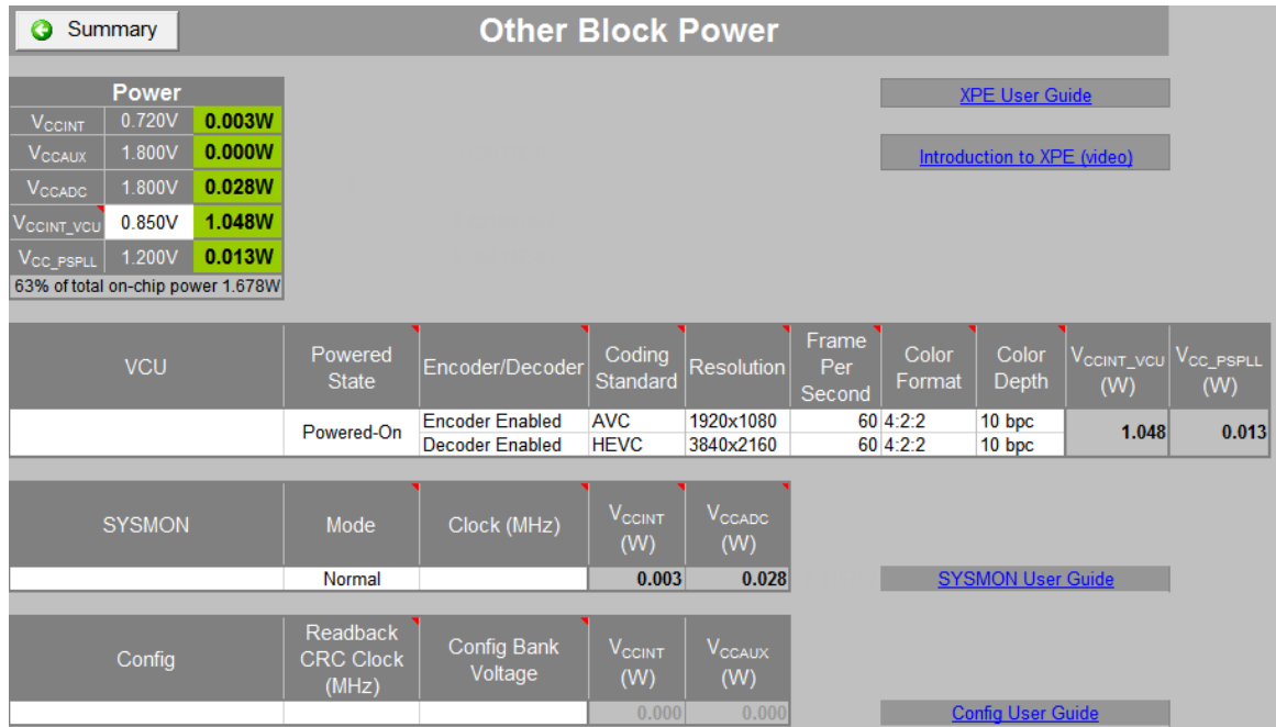
Figure 42: Other Sheet Displaying the VCU Power Estimator
