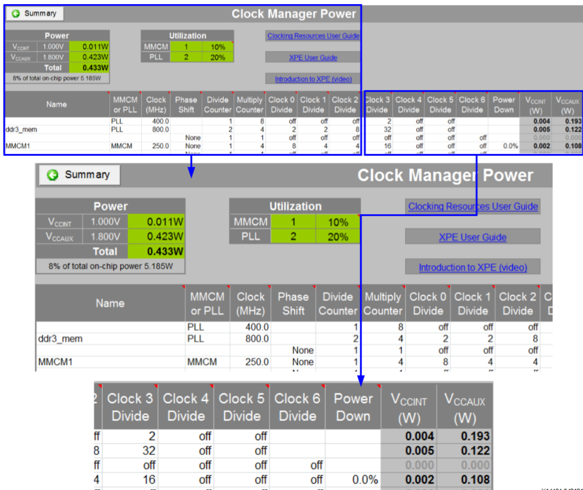
Figure 13: Clock Manager Power Sheet (7 Series Devices)
