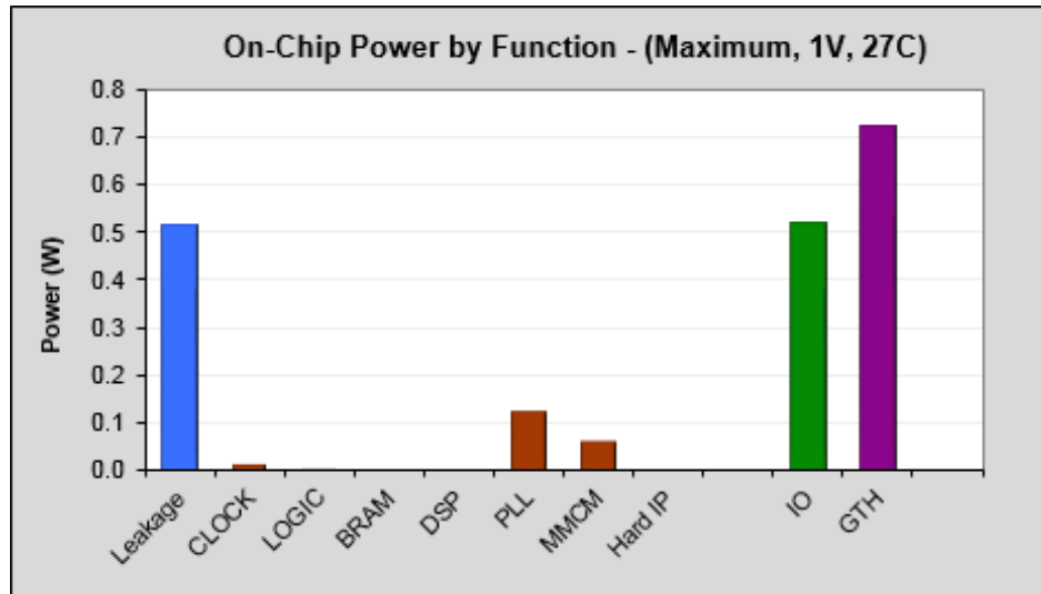
Figure 51: Graph Displaying On-Chip Power by Function
