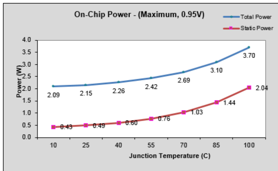
Figure 55: Graph Displaying the On-Chip Power Variance with Respect to Junction Temperatures
