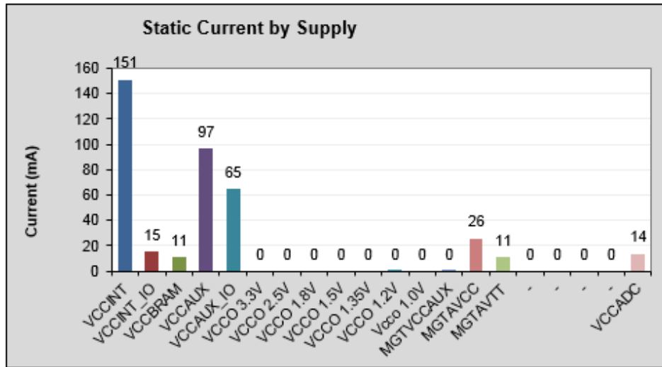
Figure 53: Graph Displaying the Static Current by Supply
