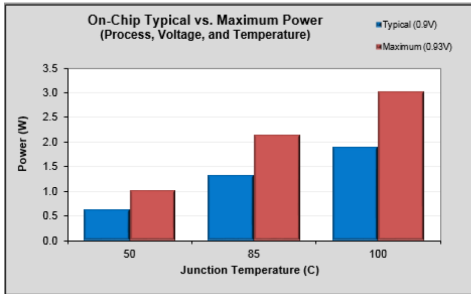
Figure 54: Graph Displaying the On-Chip Typical vs Maximum Power Variance
