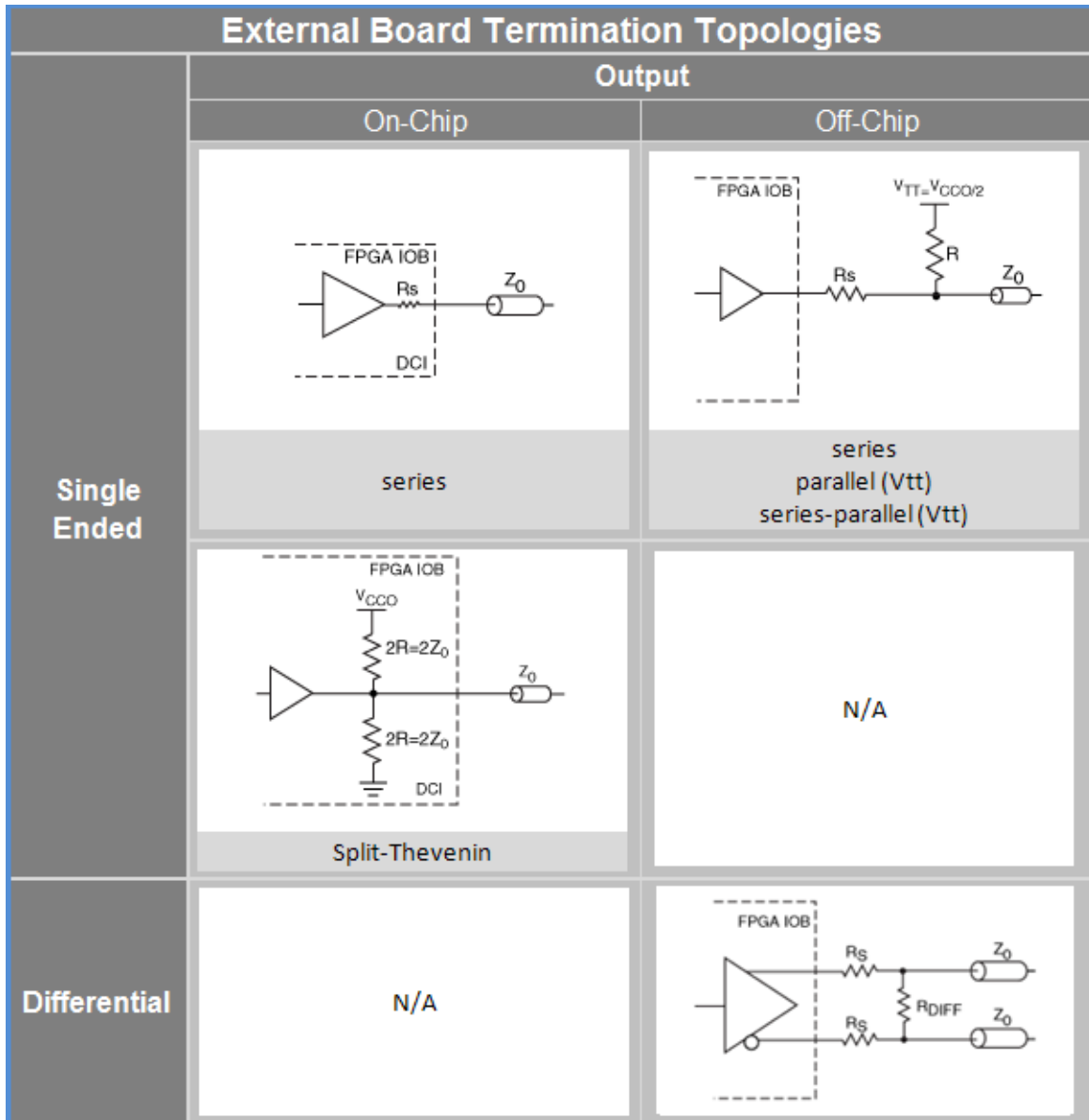
Figure 20: External I/O Termination Topologies (Virtex-6 and 7 Series Devices)
